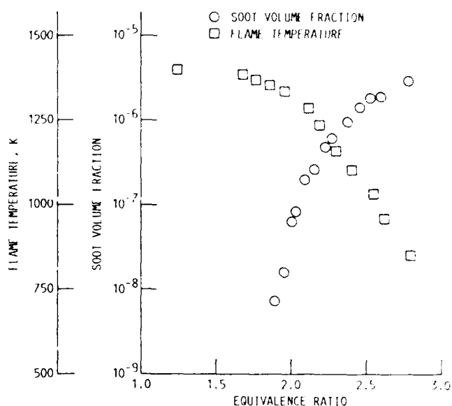
Figure 9.—Soot volume fractions and flame temperatures as functions of equivalence ratio. Height above burner, 15 mm; cold gas velocity, 3.4 cm/s.
