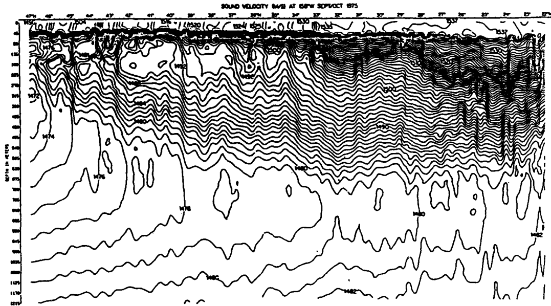
Fig. 3. A meridional section of sound speed in the Northeast Pacific. Contour intervals are at 1 \text{ m s}^{-1} . We thank Roden for permission to use his figure.
