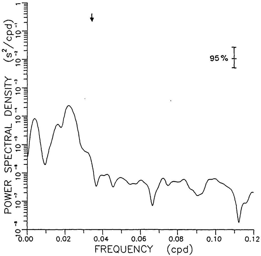
Fig. 9. The power spectral density of acoustic travel time change for the 11.7° ray traveling through the eddy field (but not the large-scale field). The arrow marks the period of mode 17, and the 95% confidence limit is shown.
