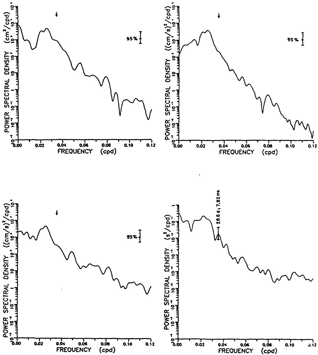
Fig. 8. Power spectral densities of sea surface displacement (upper left) and meridional currents in the upper and lower layers (lower left and upper right) at station 1 and acoustic travel time change for the 11.7^\circ ray (lower right) computed over the 4-year record. In the travel time figure, the period and rms travel time of mode 17 are labeled. In the other figures, the arrow marks the period of the mode. The 95% confidence limits are shown.
