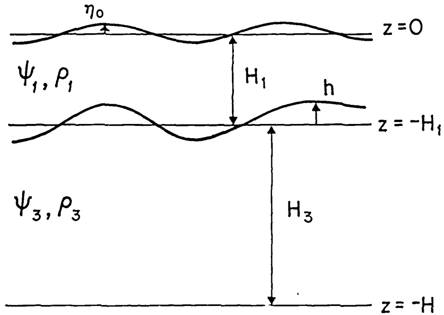
Fig. 1. Definition figure of the quantities computed in the quasi-geostrophic model. The undisturbed depth is H and the undisturbed layer thicknesses are H_1 (1000 m) and H_3 (4000 m). The interface displacement is h and the surface displacement is \eta_0 (both positive up). The streamfunction in the upper and lower layers is \psi_1 and \psi_3 , respectively. The densities in the layers are \rho_1 and \rho_3 .
