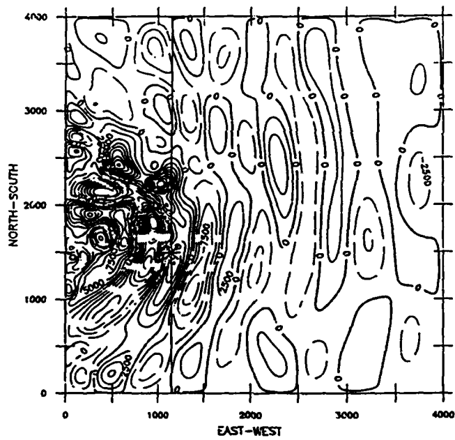
Fig. 5. Upper : Map of the upper layer streamfunction on day 4. The solid line indicates the position of the tomographic section ( x=1160 km) and the asterisk marks the location of station 1 where the sea surface elevation and currents are computed ( y=1500 km). Contour interval is 1 \times 10^4 \text{ m}^2 \text{ s}^{-1} and the dashed lines correspond to negative values. Bottom : Same except for the lower layer. The contour interval is 0.25 \times 10^4 \text{ m}^2 \text{ s}^{-1} .
