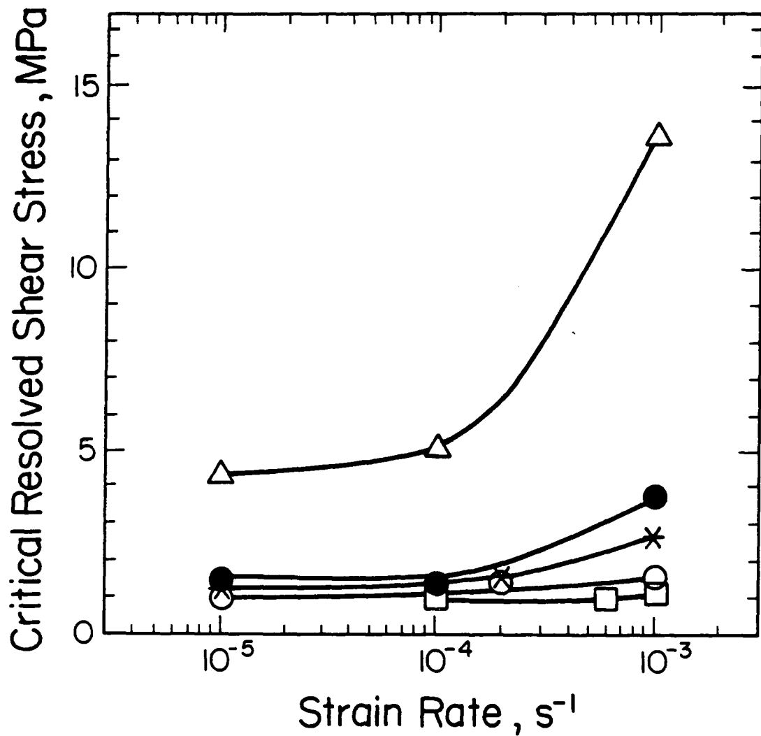
Figure 5. Variation of CRSS with strain rate for undoped GaAs (crystal A) at different temperatures. Open triangle: 500°C; solid circles: 700°C; asterisk: 900°C; open circles: 1100°C; open squares: 1150°C.
