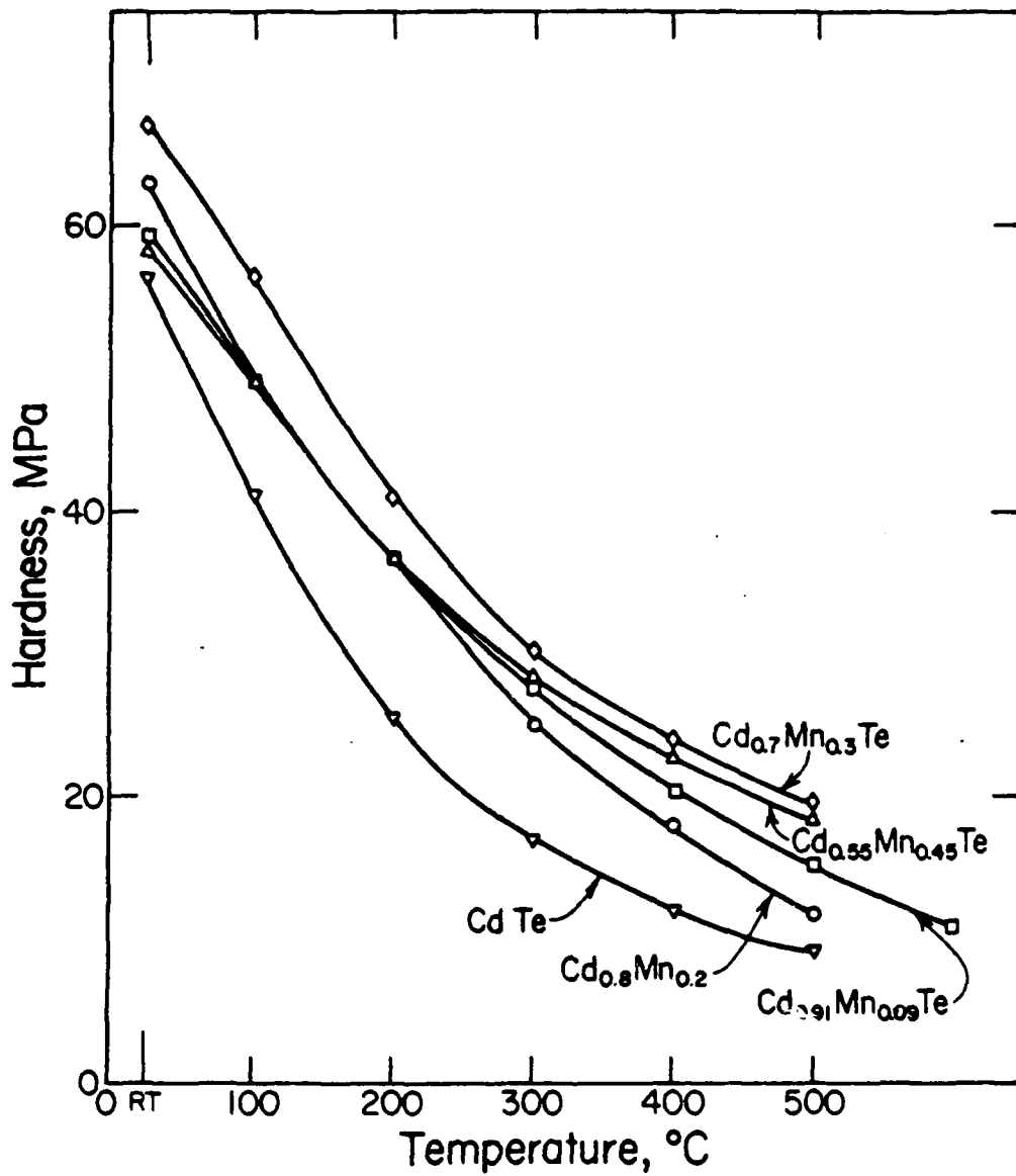
Figure 7. Vickers hardness versus temperature for Cd_{1-x}Mn_xTe for 0 < x < 0.6 .
