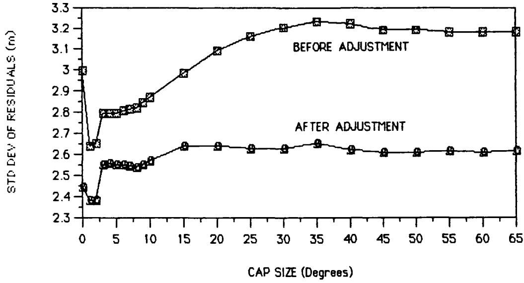
FIG 18. WEST INDIES. STANDARD DEVIATIONS OF GEIOD UNDULATION RESIDUALS.
