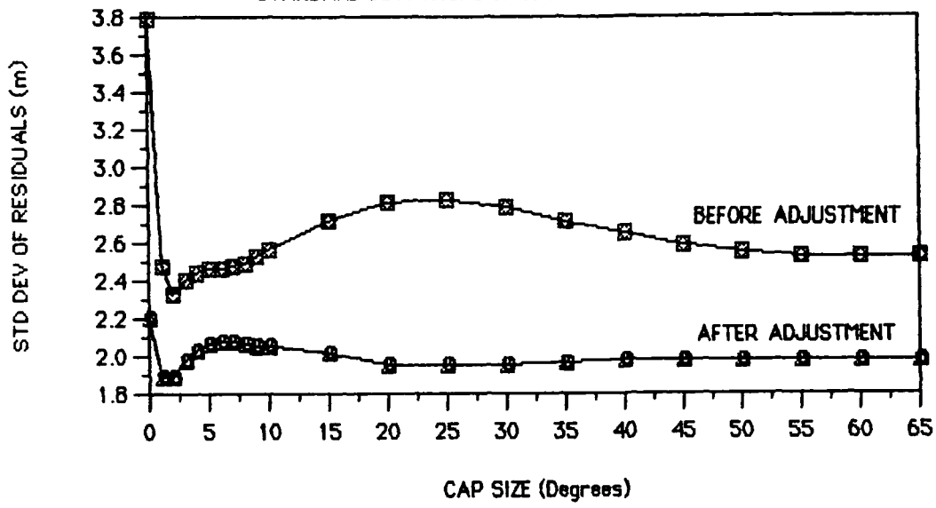
FIG 4. ALASKA. STANDARD DEVIATIONS OF GEOID UNDULATION RESIDUALS.
