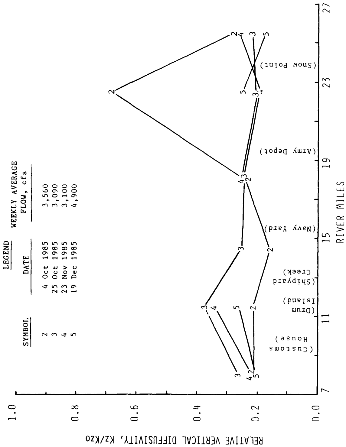
Figure A21. Vertical mixing parameter K_z/K_{z0} for fall 1985 survey
