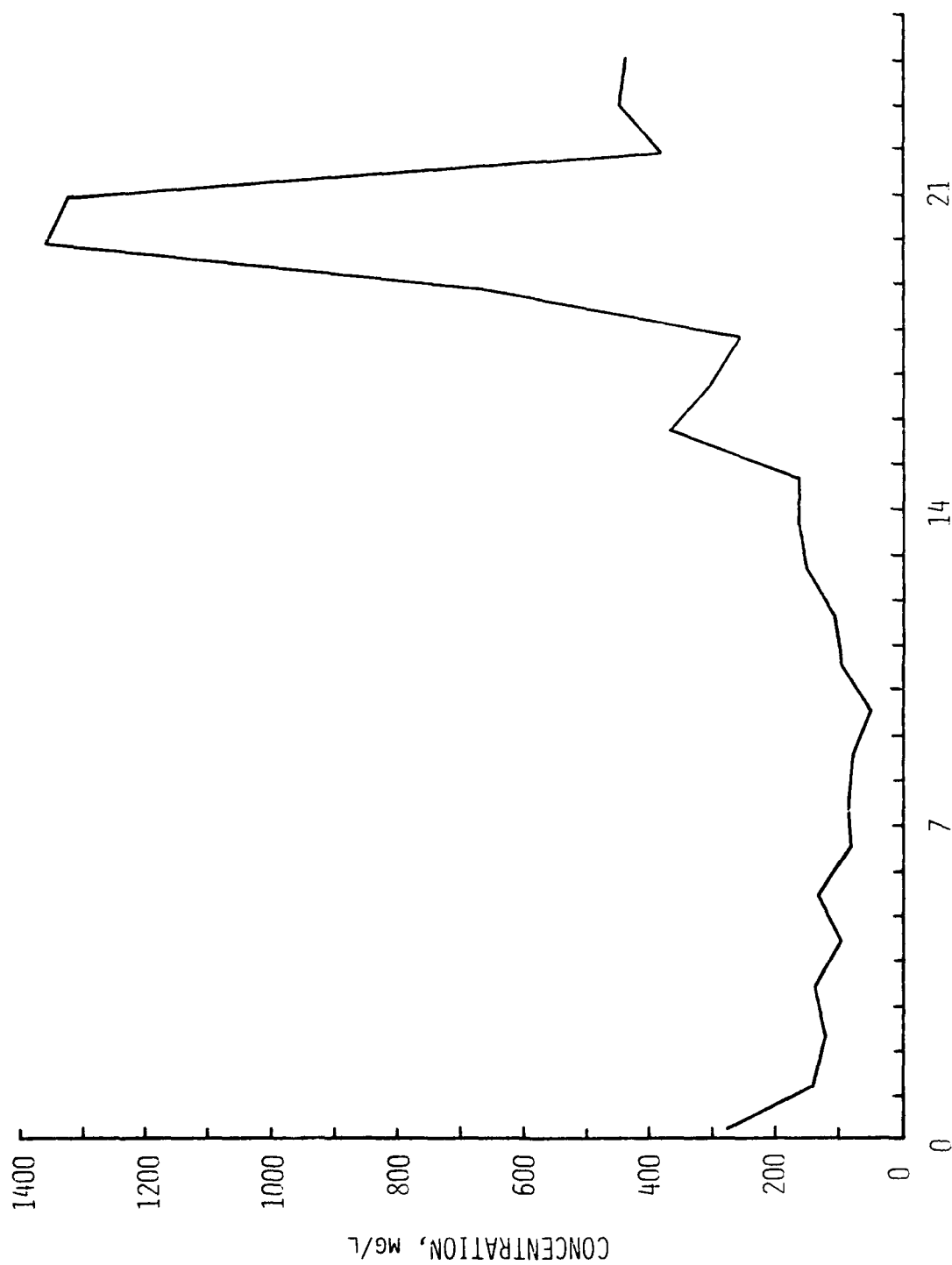
Figure A22. Daily tidal-averaged suspended sediment concentration at sta 2, 0.75 depth (see Figure A23 for tidal conditions)
