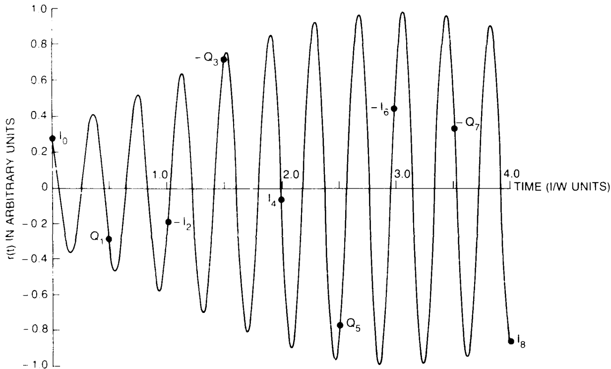
Fig. 1 - Sine wave modulated by Gaussian pulse. Sample points are labeled with corresponding I_n , Q_n values.
