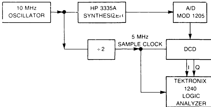
Fig. 6 — Test instrumentation
