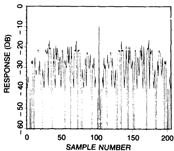
Fig. 13 — Aperiodic ACF of the quadratic residue code, p = 103
