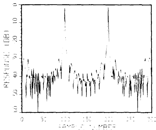
(c) f_d T = 0.25
