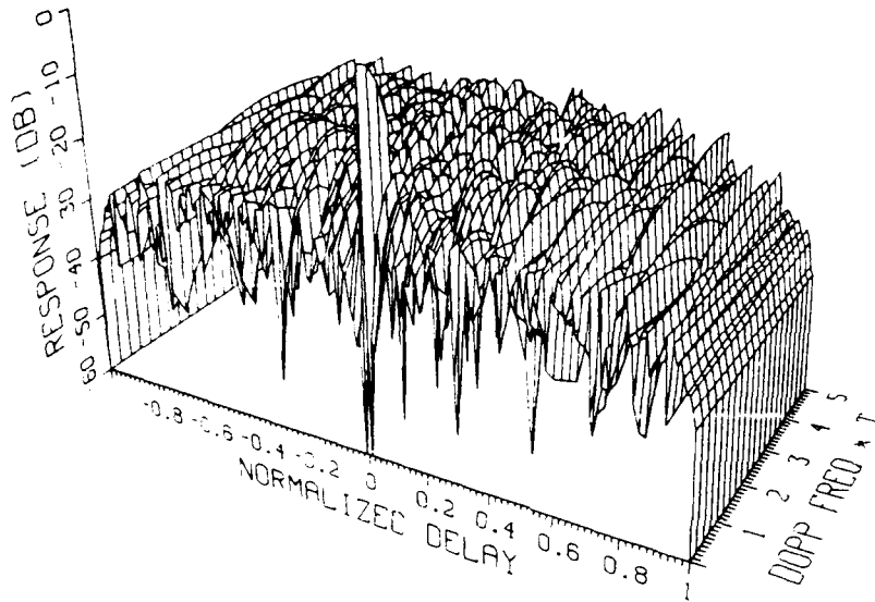
Fig. 8 — Ambiguity function of the primitive root code ( p = 101 , \alpha = 2 )
