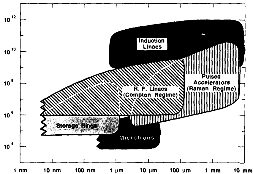
Figure 2. FELs for different wavelength regimes use different accelerator technologies. The FEL resonance equation states that wavelength depends inversely as the square of the electron energy. Thus, low-voltage machines such as diode pulsers and electrostatic accelerators are generally used for the far-infrared and millimeter wave regions. To reach shorter wavelengths, higher electron energy with high beam brightness is required. Storage rings and rf linacs with advanced injectors appear capable of extending FEL operation to 100 nm and below.
