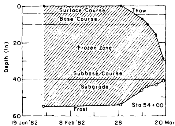
Figure 16 (cont'd). Variation of resilient stiffness with frozen zone change, station 54+00.
