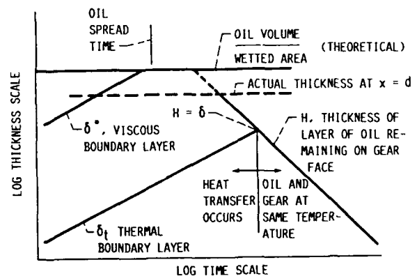
FIGURE 2. - CHARACTERISTIC LENGTH AND TIME SCALES FOR OIL FILM ON ROTATING GEAR TOOTH.
