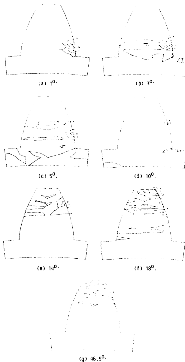
FIGURE 6. - TEMPERATURE RISE CONTOURS (IN DEGREES CELSIUS) AT 1^{\circ} TO 46.5^{\circ} OF GEAR ROTATION AFTER INITIAL TOOTH CONTACT. INITIAL NONEQUILIBRIUM CONDITIONS WITH 10 EQUAL PREASSIGNED FIXED CONTOUR LEVELS BETWEEN MINIMUM AND MAXIMUM TEMPERATURE. SPEED 10 000 RPM; LOAD 5912 N/CM (3378 LB/IN.); 87.5 PERCENT OIL JET IMPINGEMENT DEPTH; NO BOUNDARY LAYER EFFECT.
