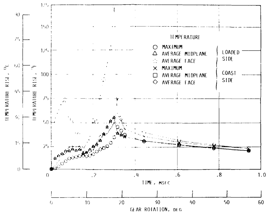
FIGURE 10. TEMPERATURE RISE VERSUS TIME AND ROTATION. INITIAL NONEQUILIBRIUM CONDITIONS. SPEED, 10 000 RPM; LOAD, 5912 N/CM (35/8 LB/IN.); 87.5 PERCENT OIL JET IMPINGEMENT DEPTH; WITH BOUNDARY LAYER EFFECTS.
