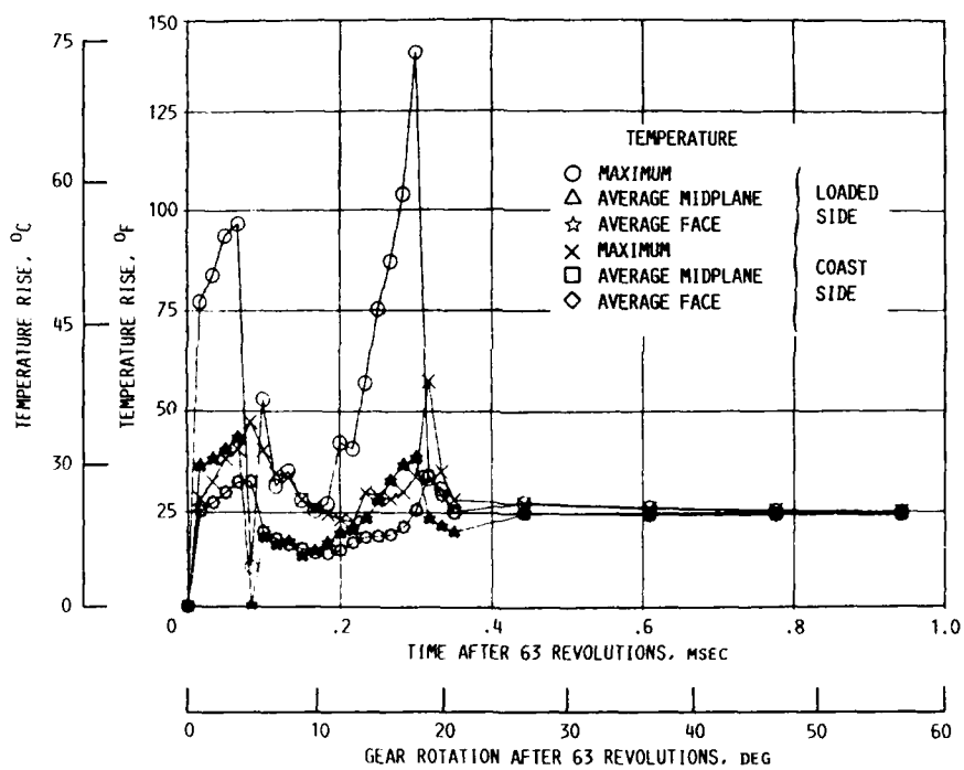
FIGURE 13. - TEMPERATURE RISE VERSUS TIME OR GEAR ROTATION AFTER 63 REVOLUTIONS. SPEED, 10 000 RPM; LOAD, 5912 N/cm (3378 LB/IN.); 87.5 PERCENT OIL JET IMPINGEMENT DEPTH; WITHOUT BOUNDARY LAYER EFFECTS AFTER STEADY-STATE EQUILIBRIUM CONDITIONS.
