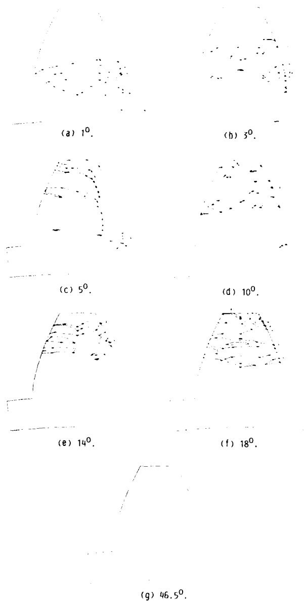
FIGURE 14. - TEMPERATURE RISE CONTOURS (IN DEGREES CELSIUS) AT 1^{\circ} TO 46.5^{\circ} OF GEAR ROTATION AFTER INITIAL CONTACT AFTER 63 GEAR REVOLUTIONS. WITH 10 EQUAL PREASSIGNED FIXED CONTOUR LEVELS BETWEEN MINIMUM AND MAXIMUM TEMPERATURE. SPEED, 10 000 RPM; LOAD 5912 N/CM (3378 LB/IN.); 87.5 PERCENT OIL JET IMPINGEMENT; WITH BOUNDARY LAYER EFFECTS.
