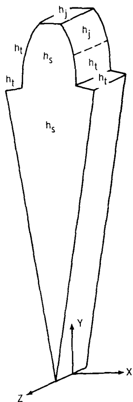
FIGURE 3. - CONVECTIVE HEAT TRANSFER COEFFICIENT ZONES.
