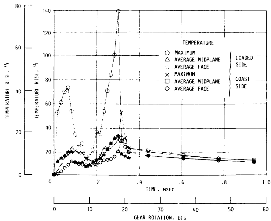
FIGURE 7. - TEMPERATURE RISE VERSUS TIME OR DEGREES ROTATION. INITIAL NONEQUILIBRIUM CONDITIONS. SPEED, 10 000 RPM; LOAD, 5912 N/CM (3328 LB/IN.); 87.5 PERCENT OIL JET IMPINGEMENT DEPTH; NO BOUNDARY LAYER EFFECTS.
