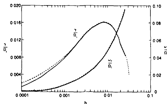
FIG. 2. The real and imaginary frequencies normalized by \Omega_i for the KH instabilities for the dc electric field profile given by E = E_0 \text{sech}^2(x/L) are plotted as a function of b . The solid lines are the eigenvalues of Eq. (29) while the dotted lines are the fluid results given in Ref. 9. Here \epsilon = 0.1 , \tau = 1 , \mu = 1837 , and u = 0.0001 .
