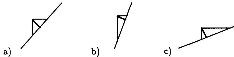
Figure 15. Approximating the normal distance to a line depending on the slope, a) y = x , b) using x component, c) using y component.
