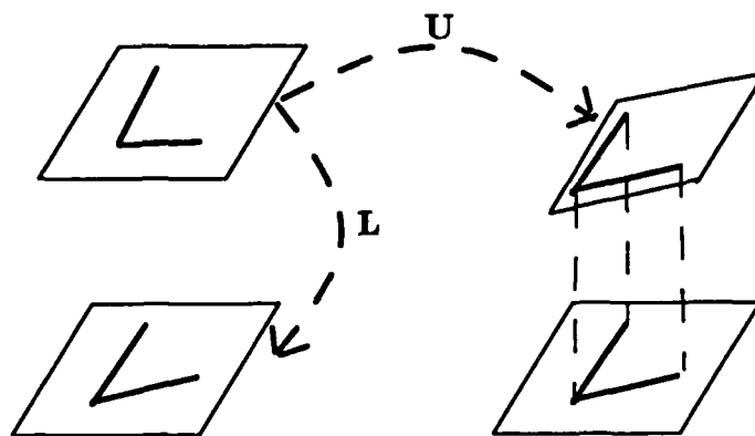
Figure 9. The geometrical interpretation of \mathbf{U} .
