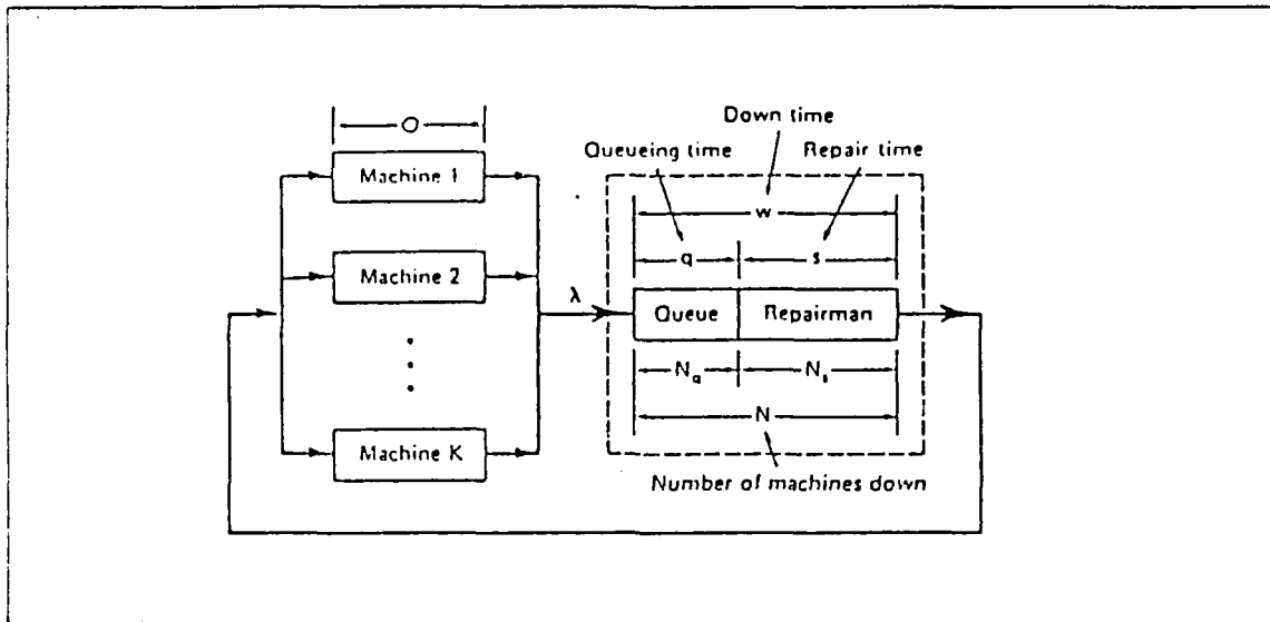
Figure 6. Queuing System with One Repairman (M/M/1/K/K)
