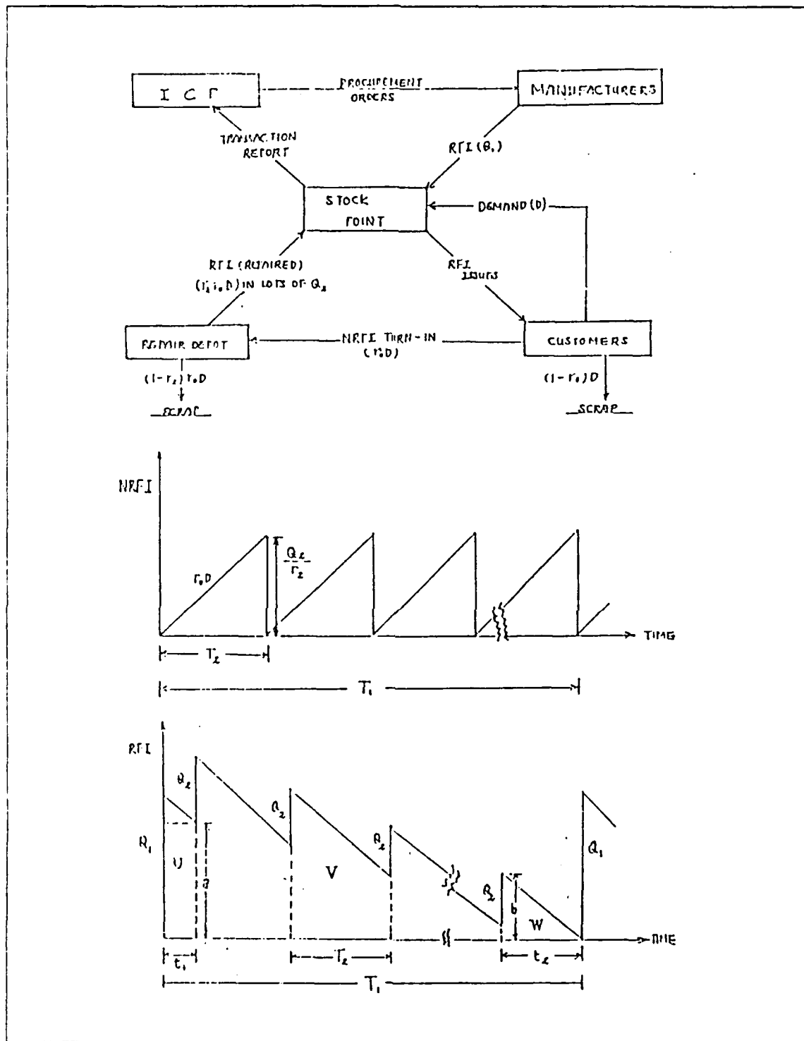
Figure 4. Repair Cycle and System for "Continuous Supplement" Model
