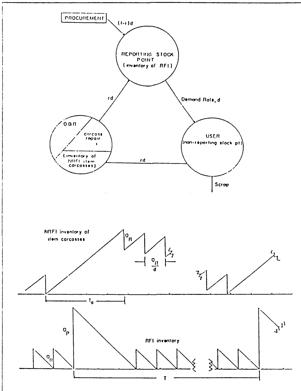
Figure 5. Repair Cycles and System for "Substitution" Model
