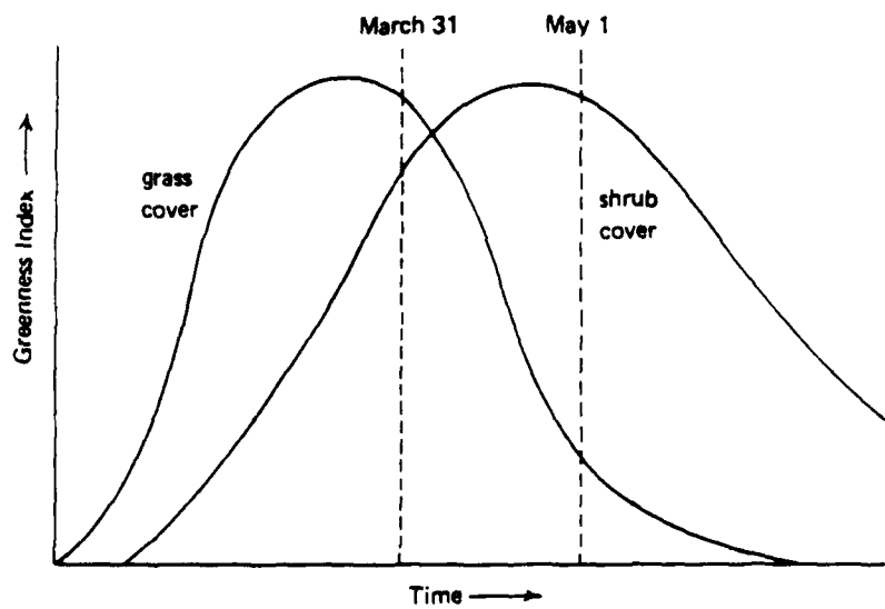
Figure 2. Conceptual representation of the phenological status of grass-dominated and shrub-dominated vegetation types in the study area. Dates are approximate for 1987.
