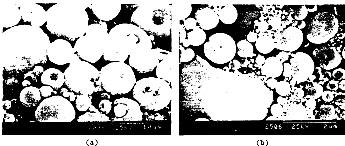
Figure 1. SEM micrographs of powders formed from (a) a \text{Ti}(\text{O-n-Bu})_4 -in-acetonitrile emulsion and (b) a \text{Ti}(\text{O-n-Bu})_4 -in-butylene carbonate emulsion.
