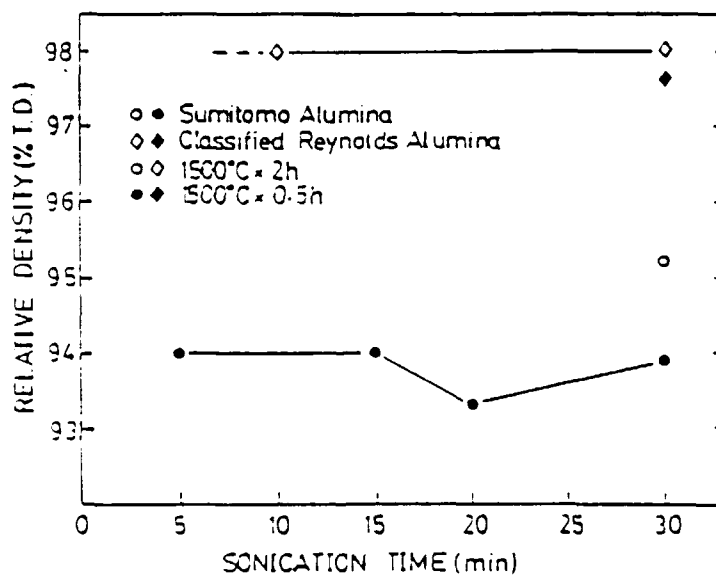
Figure 4. Relative density versus sonication time for \text{Al}_2\text{O}_3 - \text{Al}_2\text{TiO}_5 samples having a starting powder composition of 20.7 wt% \text{TiO}_2 , using Sumitomo and classified Reynolds \text{Al}_2\text{O}_3 and sintering conditions of 1500^\circ\text{C} for either 0.5 or 2.0 h.
