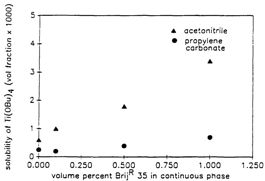
Figure 11. Solubility of \text{Ti}(\text{O-}n\text{-Bu})_4 in acetonitrile and propylene carbonate as a function of Brij ® 35 concentration.
