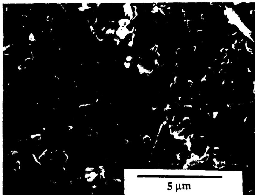
Figure 6. SEM of the fracture surface of a composite containing 8 vol% Lonza SiC powder after sintering for 60 min at 1500°C.
