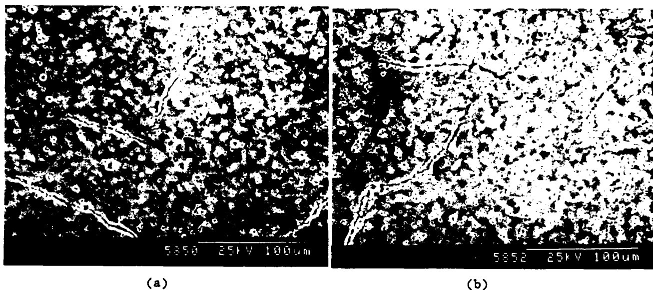
Figure 3. SEMs of polished surfaces of \text{Al}_2\text{O}_3 - \text{Al}_2\text{TiO}_5 samples made with Sumitomo \text{Al}_2\text{O}_3 and a) 0.2 wt% or b) 1.0 wt% polyvinyl alcohol, fired at 1500^\circ\text{C} for 0.5 h.
