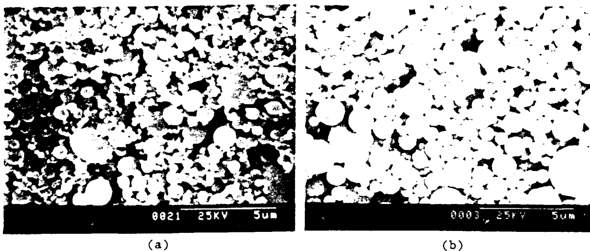
Figure 2. SEM micrographs of powders formed from (a) a \text{Ti}(\text{O-n-Bu})_4 -in-propylene carbonate emulsion and (b) a \text{Ti}(\text{O-n-Bu})_4 -in-formamide emulsion.
