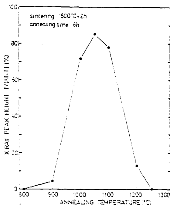
Figure 6. Decomposition ratio of \text{Al}_2\text{TiO}_5 in an \text{Al}_2\text{O}_3\text{-Al}_2\text{TiO}_5 sample versus annealing temperature and annealing time.
