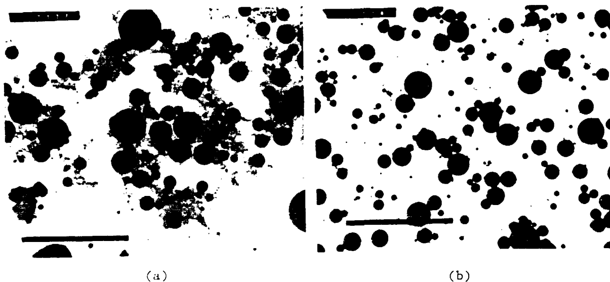
Figure 14. TEM micrographs of powders prepared from (a) a 0.5% vol% and (b) a 20 vol% \text{Al}(\text{O-sec-Bu})_3 (with 20 vol% hexane)-in-propylene carbonate emulsion (each bar = 5.0 \mu\text{m} ).
