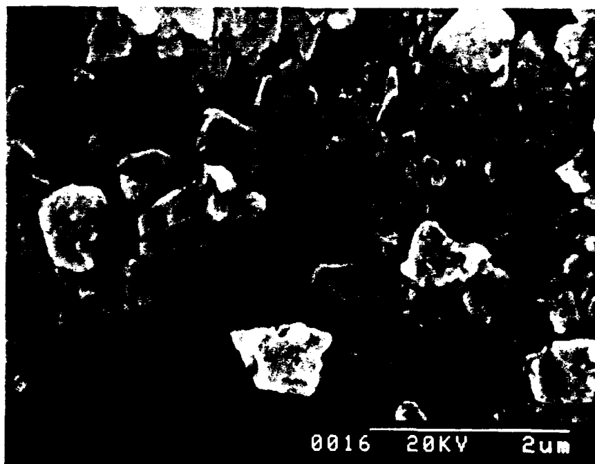
Figure 8. a) Particle-size distribution of Cut 3 ( 0.5\text{-}0.8 \mu\text{m} ), with b) accompanying photomicrograph.
