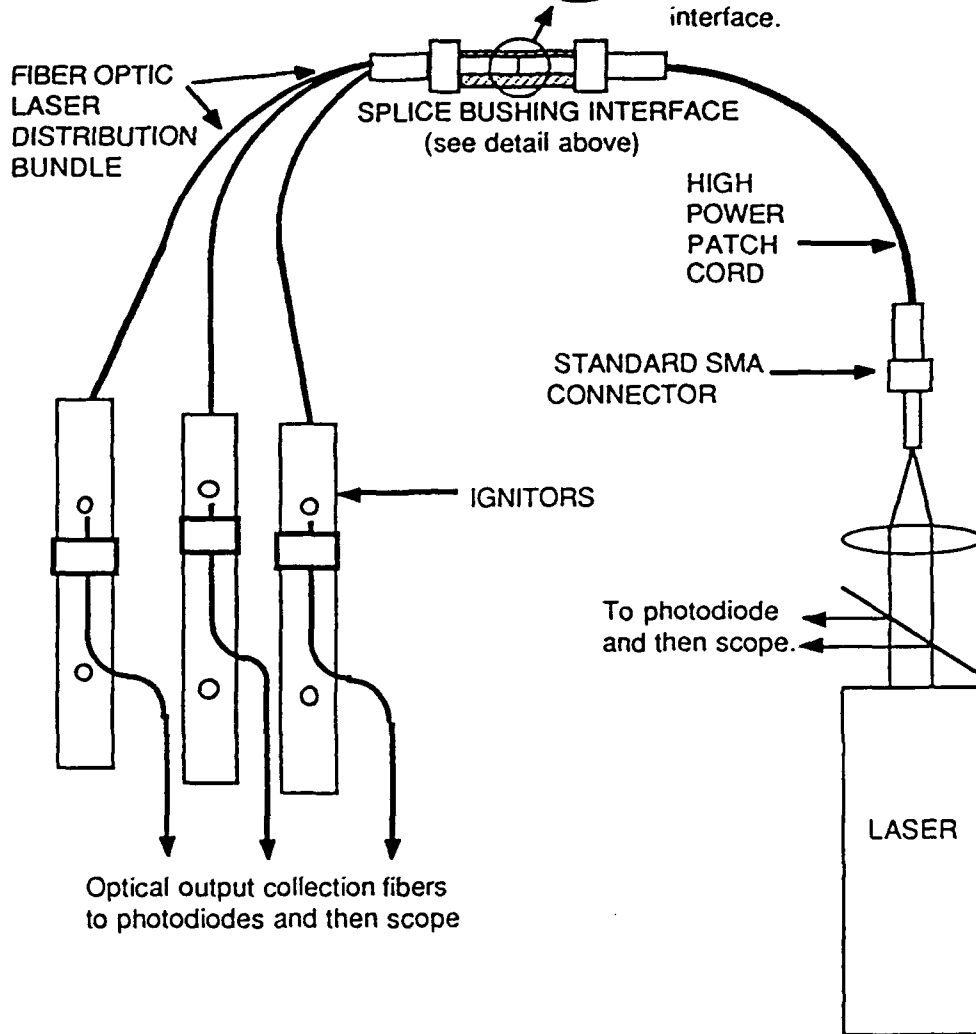
Figure 20. Simultaneity test setup
