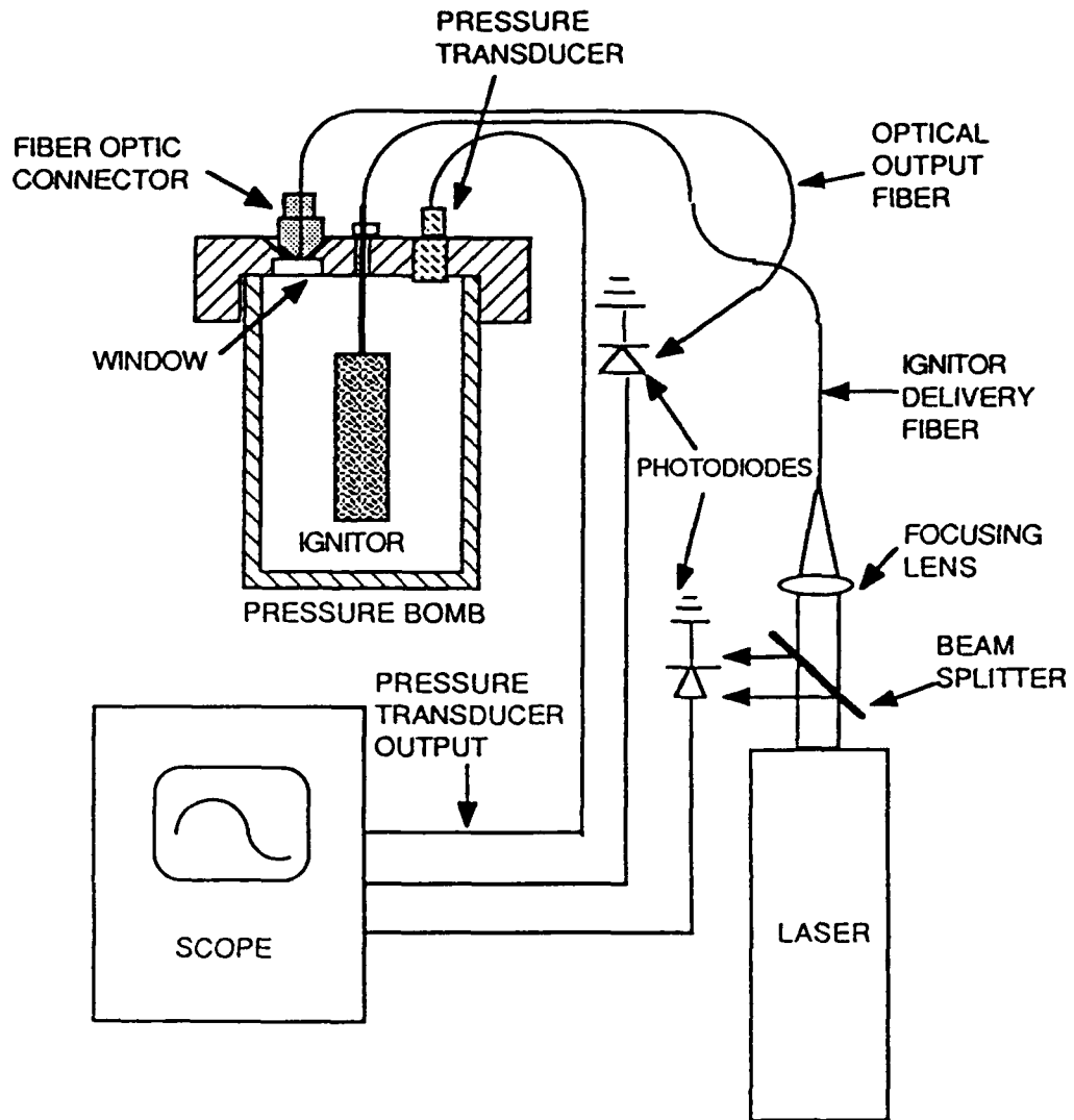
Figure 18. Test setup
