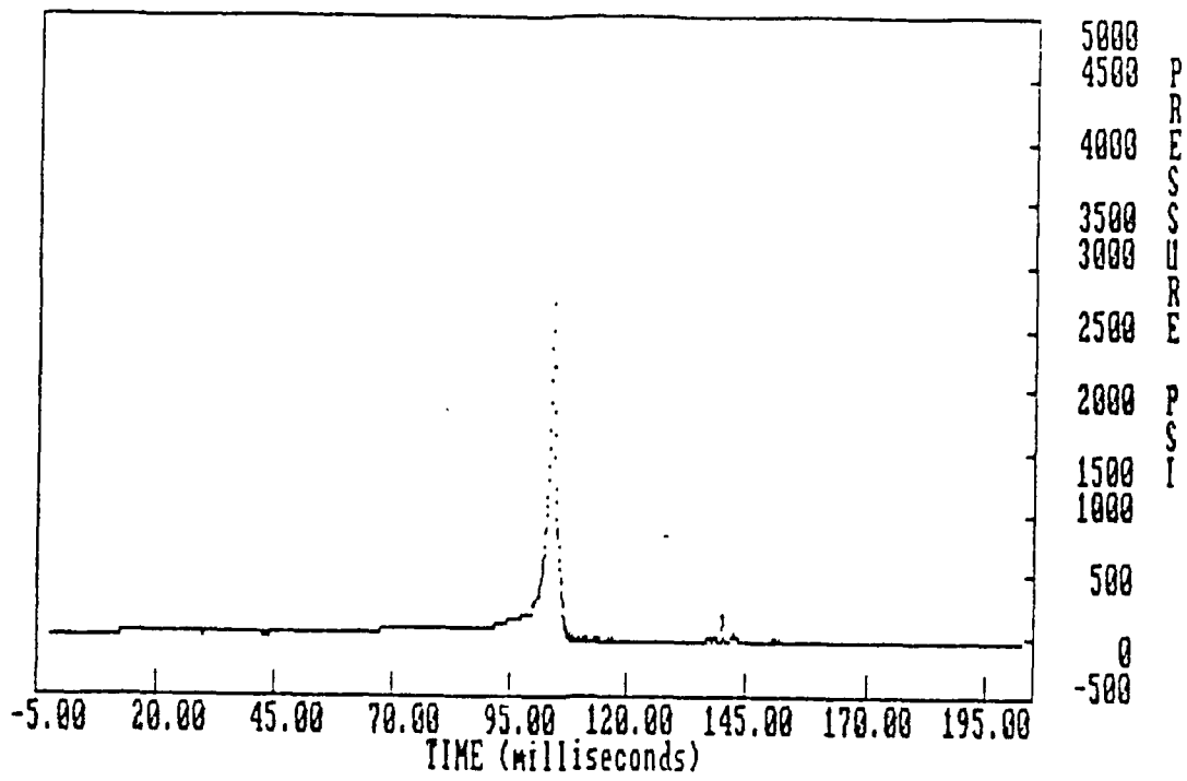
Figure 56. Live test, configuration 1 front pressure transducer
