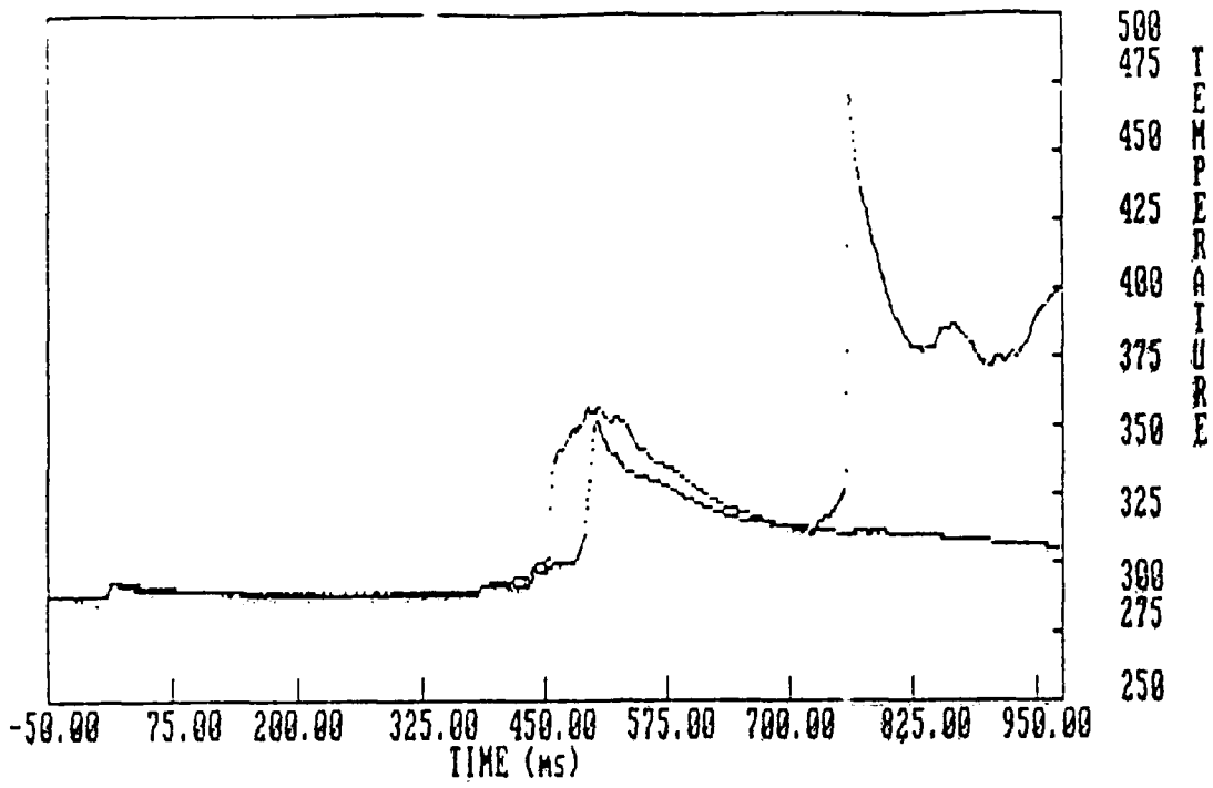
Figure 52. Inert test, configuration 4 both thermocouples
