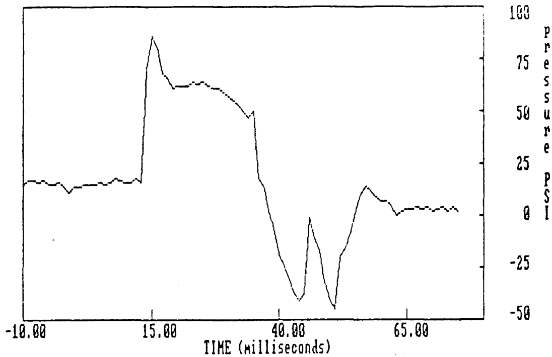
Figure 44. Inert test, configuration 3 pressure differential (rear-front)
