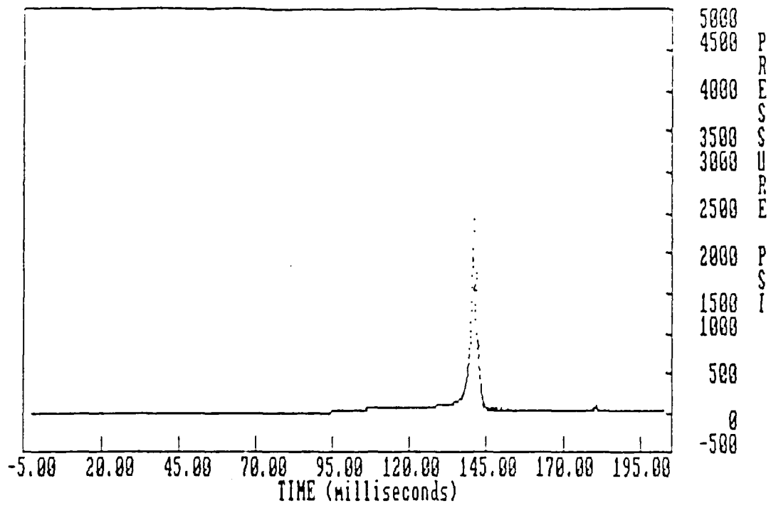
Figure 62. Live test, configuration 2 rear pressure transducer
