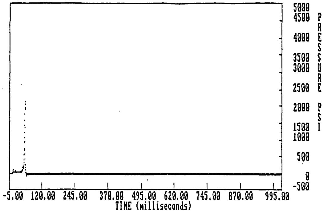
Figure 70. Live test, configuration 4 both pressure transducers
