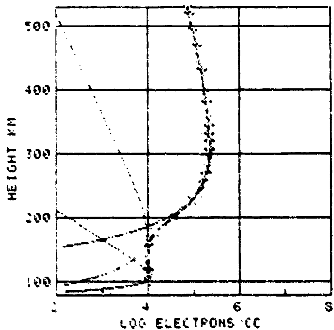
ELECTRON DENSITY PROFILE CHING-CHIU (1972)
