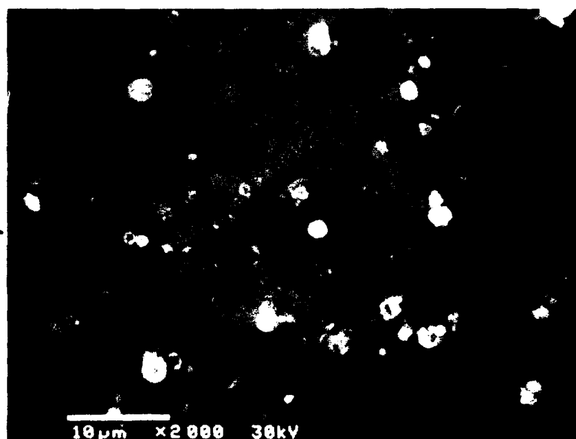
b. Iron coupon exposed to 100-neutral oil containing water and \text{SO}_2
