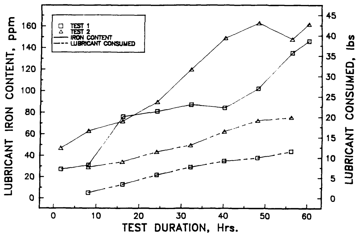
Figure 4. Iron buildup in the lubricant and the consumption of lubricant during the Petter engine wear tests
