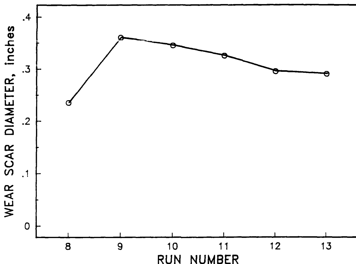
Figure 12. Wear-scar diameters plotted for Run Nos. 8 through 13 (Data given in TABLE 18; Run No. 8 = base oil; Run Nos. 9 through 13 = oil is contaminated with the same amounts of \text{SO}_2 and water)
