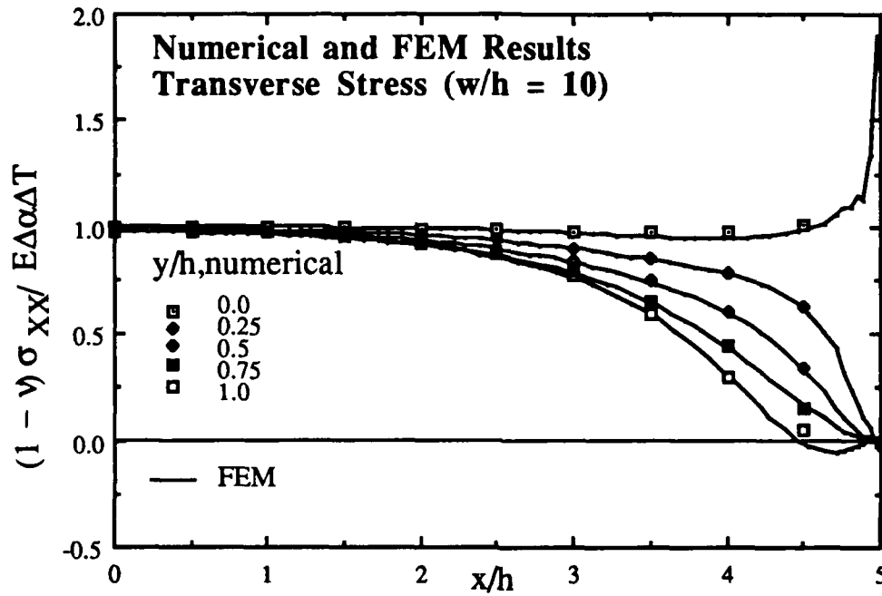
Figure 2. A comparison of numerical and FEM results for the plane stress case, showing the transverse stress in a line of w/h \approx 10 aspect ratio. The numerical results are those of Blech and Levi [3].
