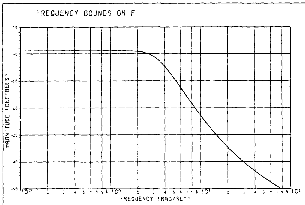
Fig. VI-5. Frequency Response of the Prefilter, f_1(j\omega)
