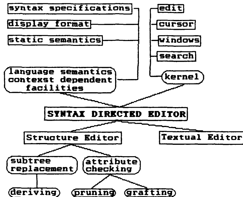
Figure 2 Cornell Synthesizer Generator
