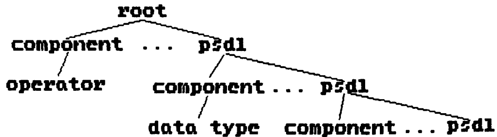
Figure 3 Derivation Tree
