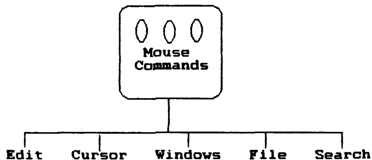
Figure 18 Mouse Commands
