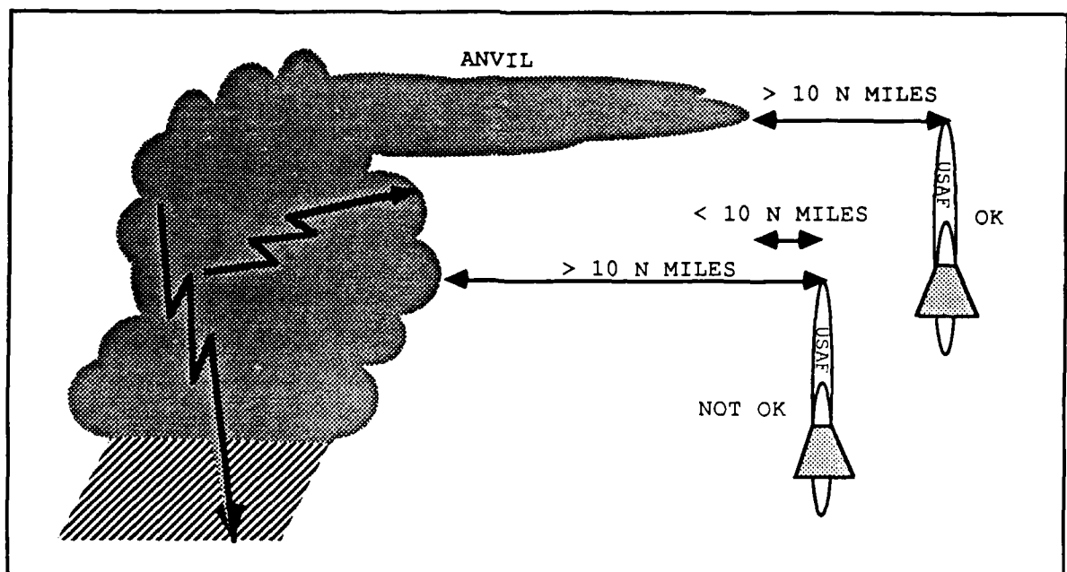
Fig 2b. Standoff Distances from Cumulonimbus and Anvils
