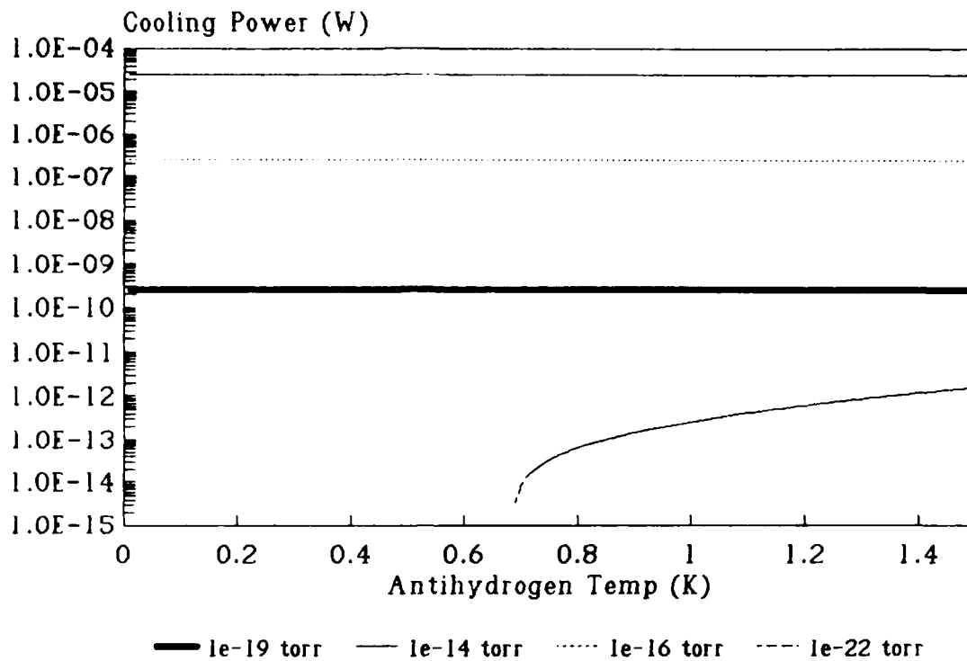
Figure IV-5. Cooling Power at Various Antihydrogen Temperatures
