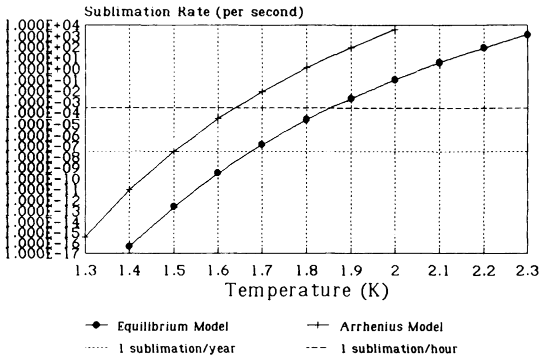
Figure II-3. Sublimation Rates in a 1-mg Solid-Hydrogen Sphere
