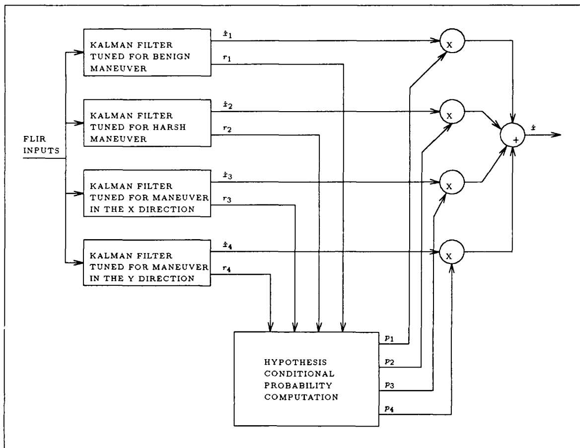
Figure 3. Multiple Model Adaptive Filter
