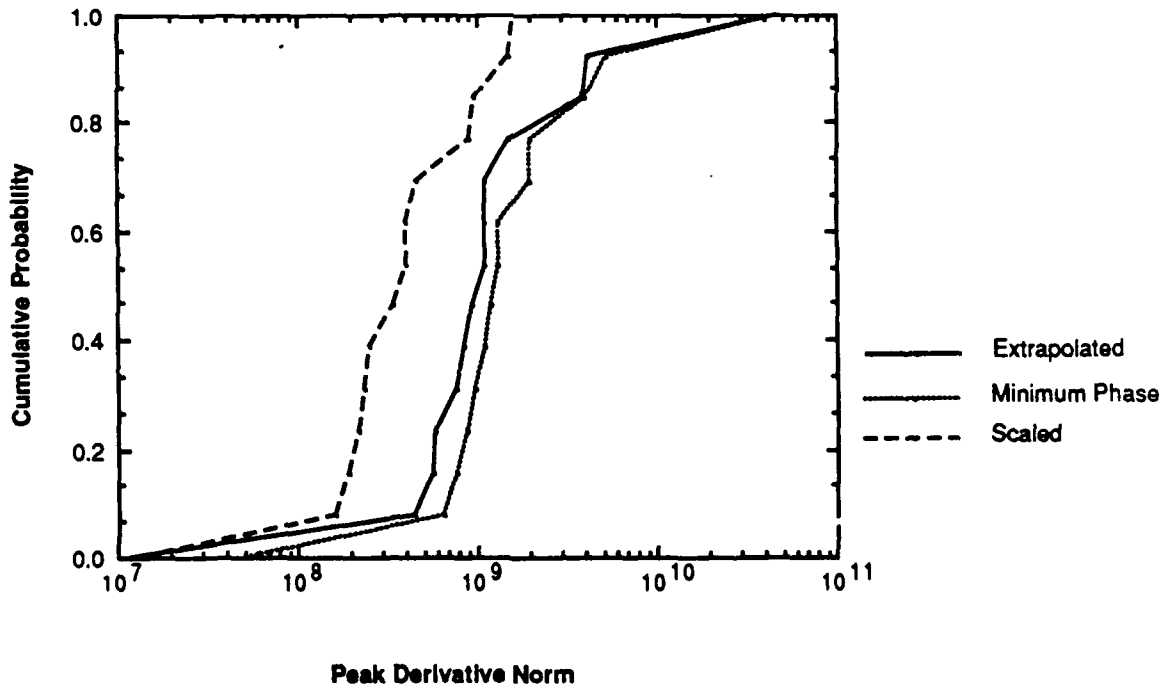
Figure C-32. Cumulative Probability Versus the Peak Derivative Norm for the 700 Series Test Points
