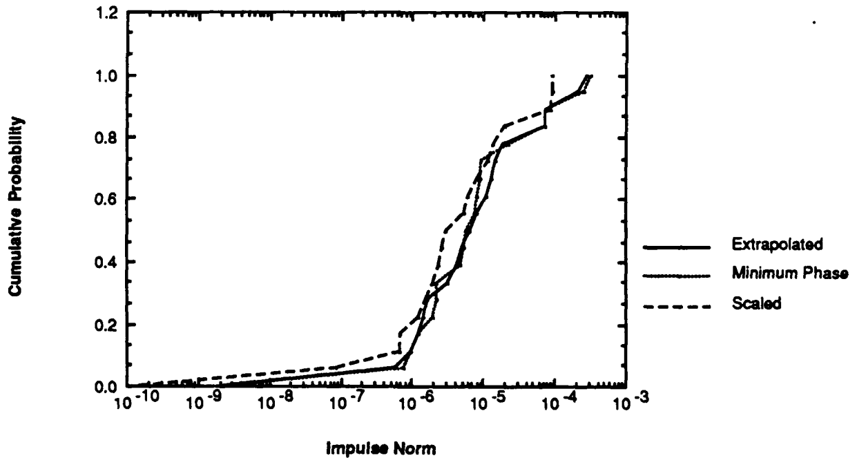
Figure C-8. Cumulative Probability Versus the Impulse Norm for the 200 Series Test Points
