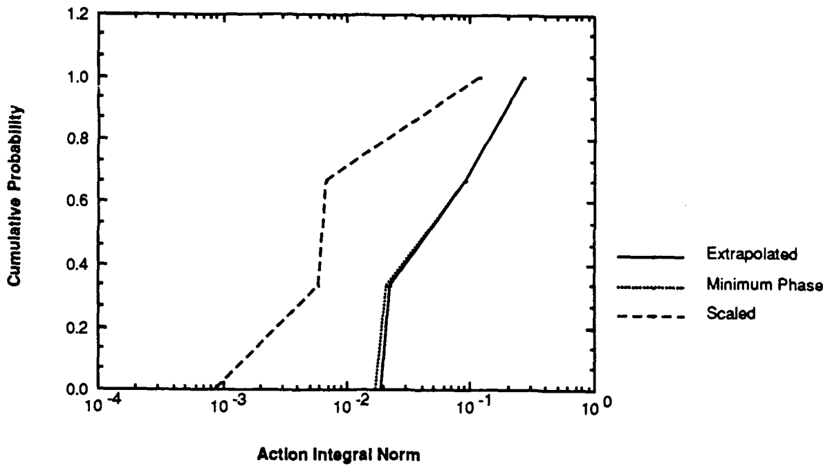
Figure C-25. Cumulative Probability Versus the Action Integral of the 500 Series Test Points
