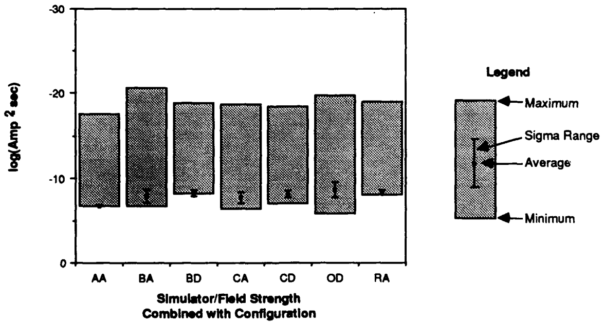
Figure 3-5. Maximum, Sigma, Average, and Minimum of the Log of the Action Integral Norm Versus Simulator and Configuration for All Test Points
