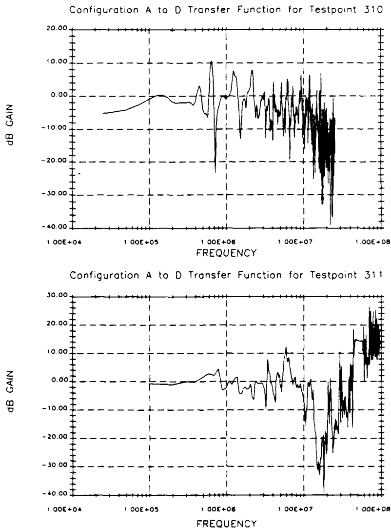
Figure 4-11. Configuration A to D Transfer Functions
