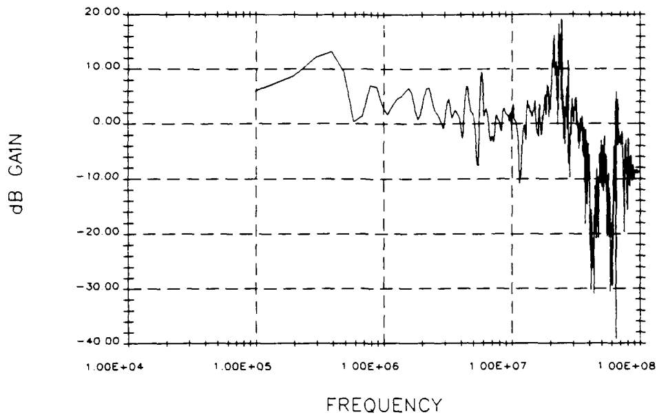
Configuration A to D Transfer Function Gain for Testpoint 407
