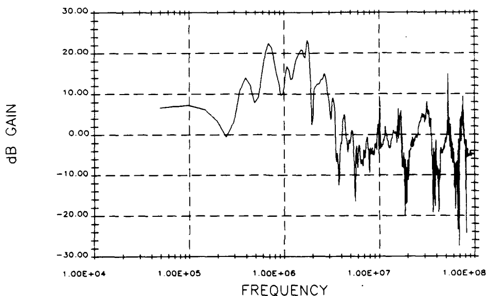
Configuration E to F Transfer Function Gain for Testpoint 325
