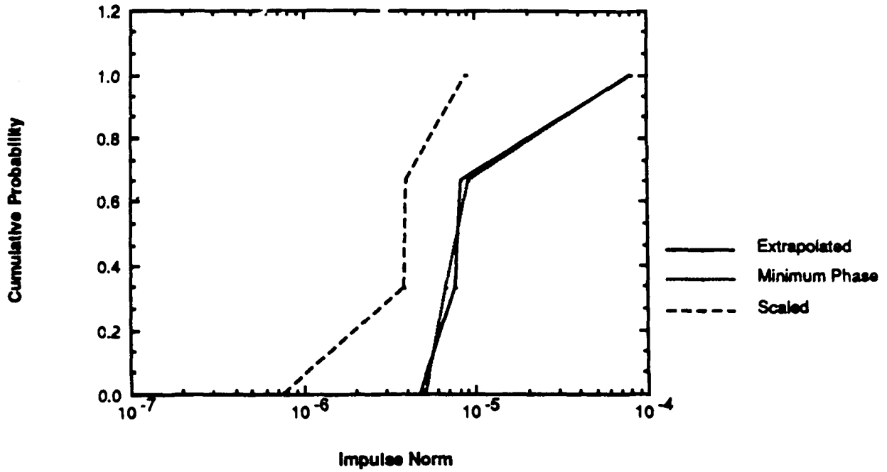
Figure C-23. Cumulative Probability Versus the Impulse Norm for the 500 Series Test Points
