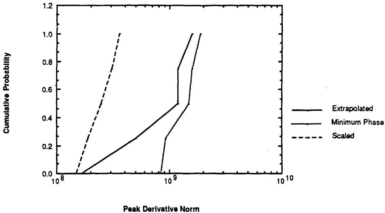
Figure C-27. Cumulative Probability Versus the Peak Derivative Norm for the 600 Series Test Points
