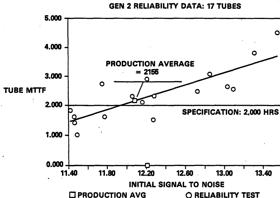
Figure 9. Correlation: Initial S/N and Tube Life
