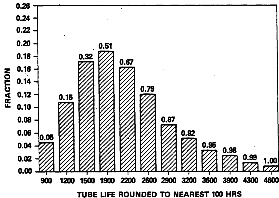
Figure 11. Second Generation Production Tube Reliability
