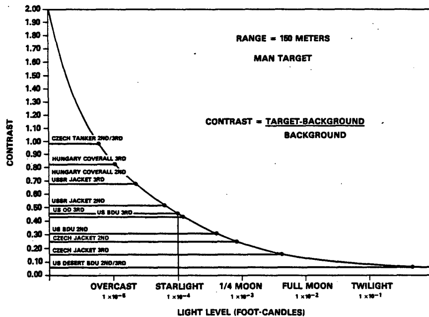
Figure 5. Contrast vs. Light Level
