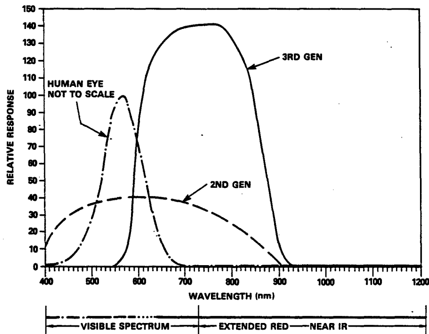
Figure 2. Detector Response
