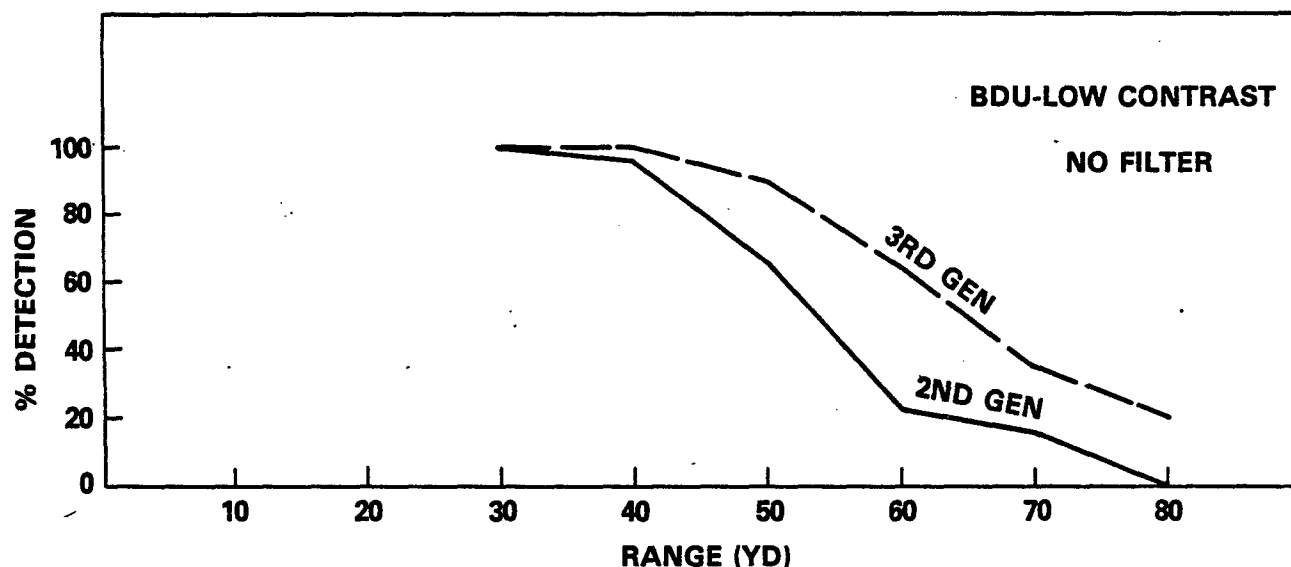
Figure 7. Range Detection Data
