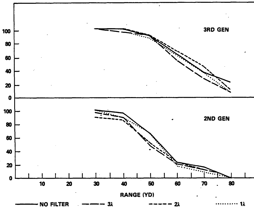
Figure 8. Range Detection Data
