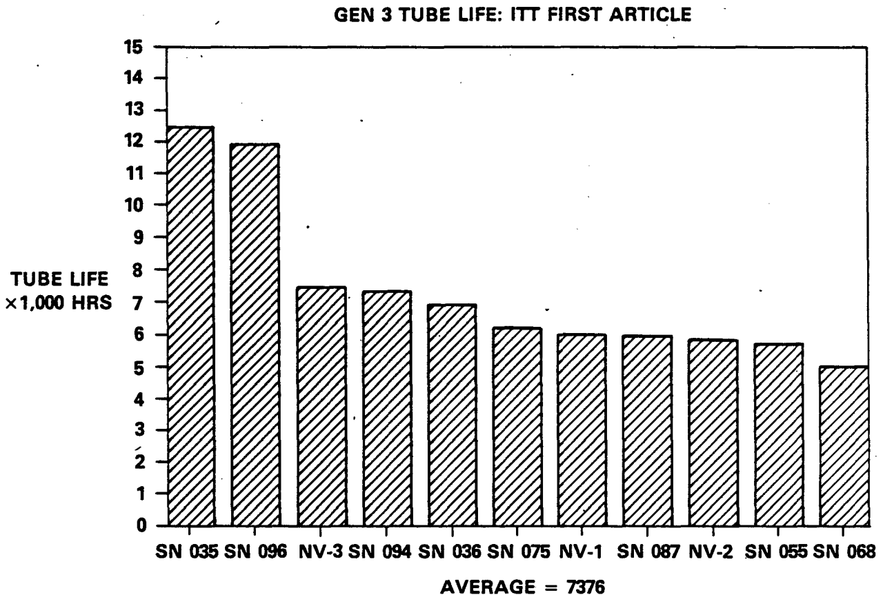
Figure 13. Third Generation Tube Life: ITT First Article
