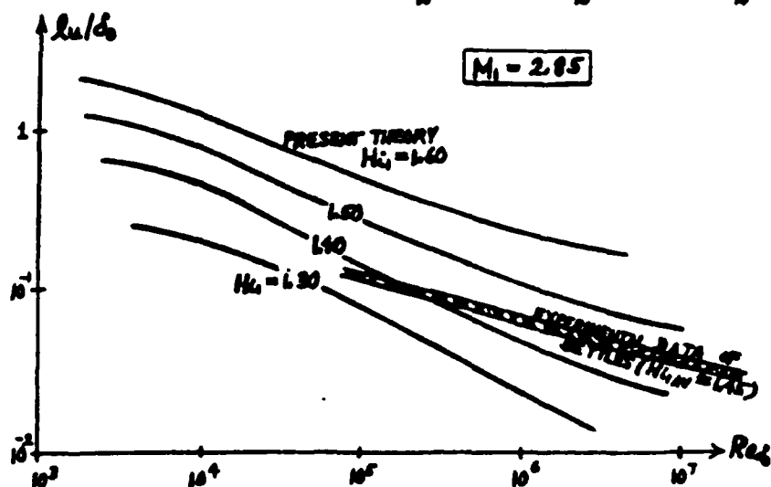
FIG. 9 Typical Shape Factor Effect on the Experimental Validation of Predicted Upstream Influence vs. Reynolds Number (Weak Compression Corners).
