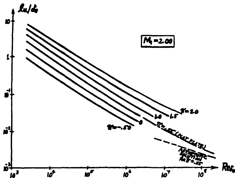
FIG. 7 Predicted Wake Factor Effect on the Upstream Influence of Non- Separating Shock-Turbulent Layer Interactions at Mach Two
