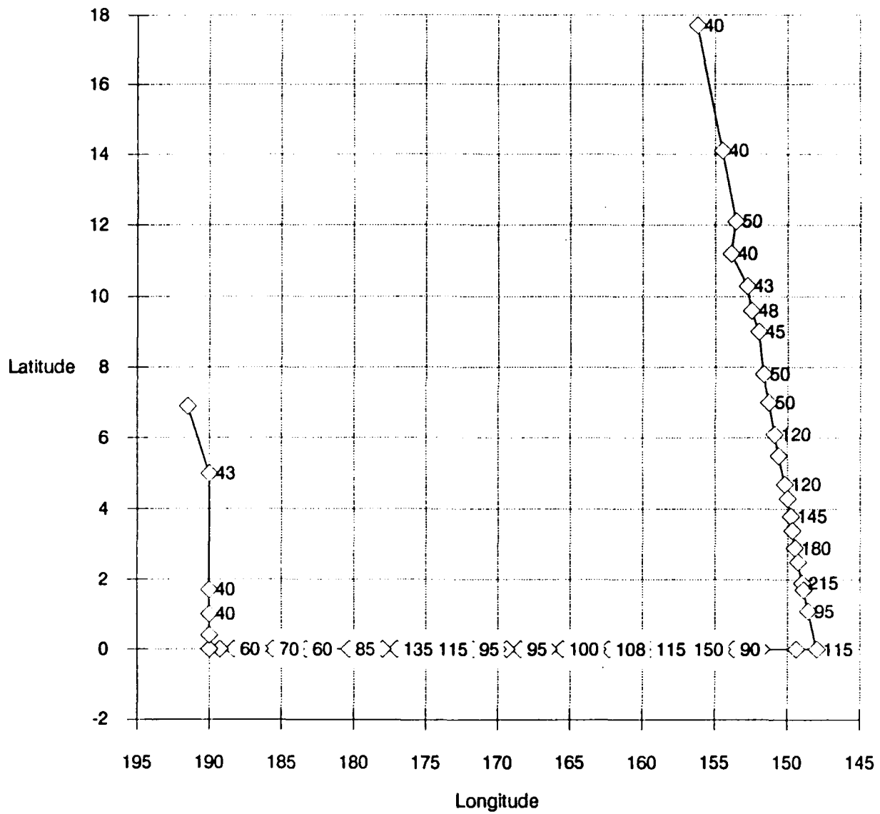
Fig. 3.1 8-21 May 1982 shiptrack of the R/V DISCOVERER with selected values of surface DMS (ng/l).
