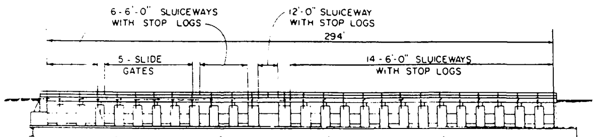
SECTION B-B
