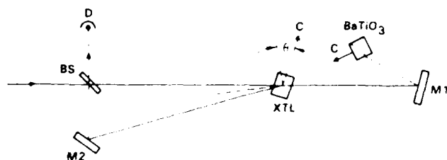
Fig. 4. Interferometer used to measure the phase shift of the phase conjugator. The light transmitted by the beam splitter, BS, and the light reflected from the self-pumped crystal of BaTiO 3 provide the pump waves for FWM in the crystal XTL. The light reflected by the beam splitter provides the probe wave. The conjugate wave and the reflection from the self pumper interfere at the detector D with a relative phase shift \phi_{01} , the phase shift of the phase conjugator.
