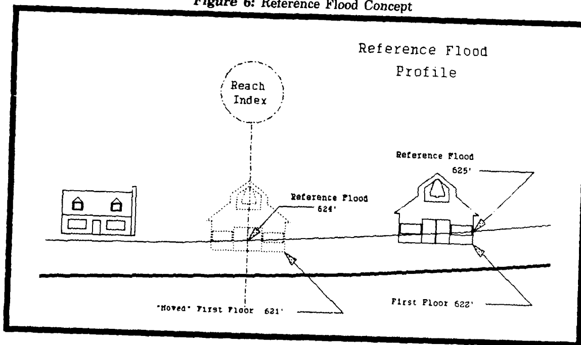
Figure 6: Reference Flood Concept
