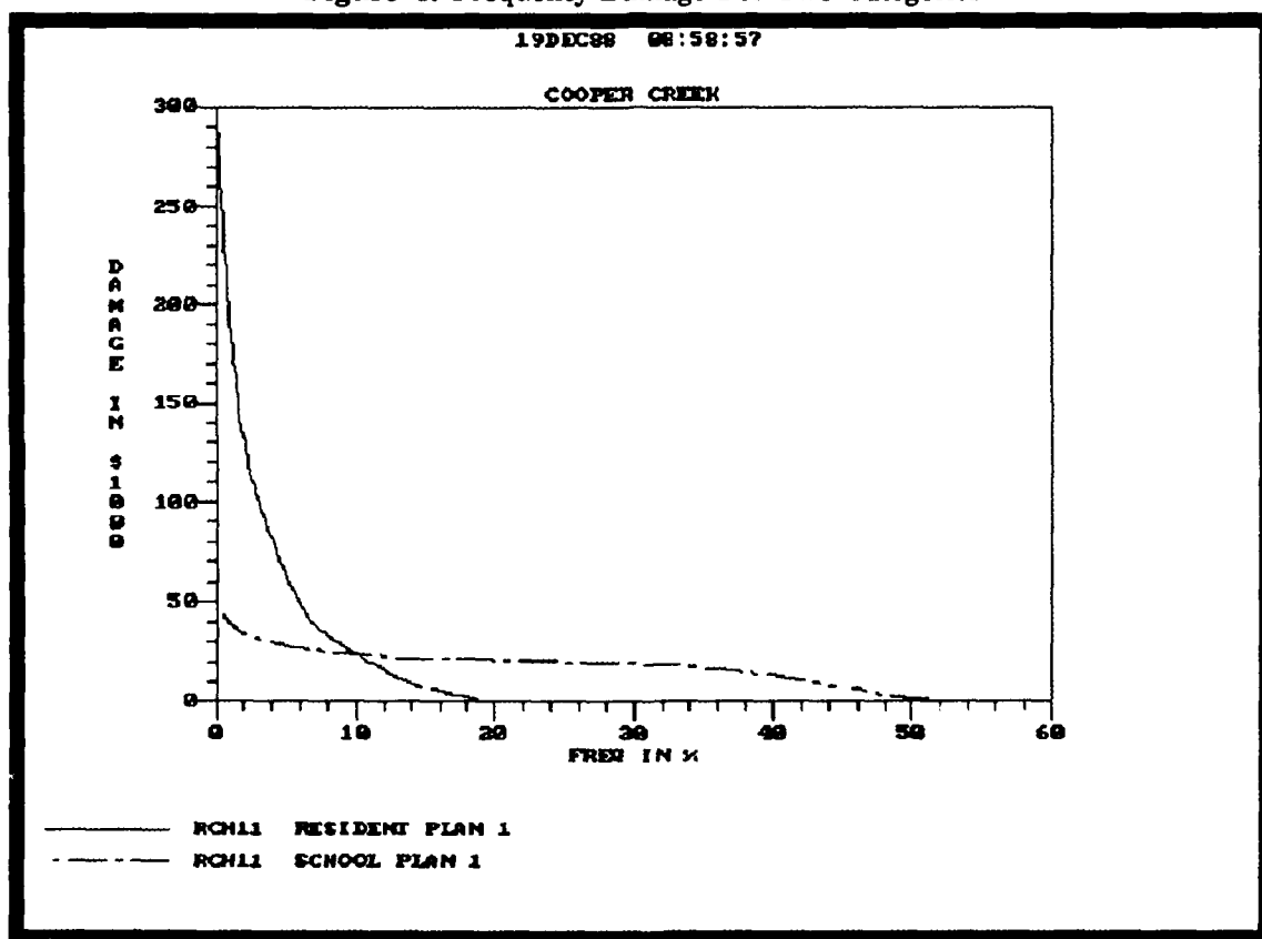
Figure 8: Frequency-Damage For Two Categories
