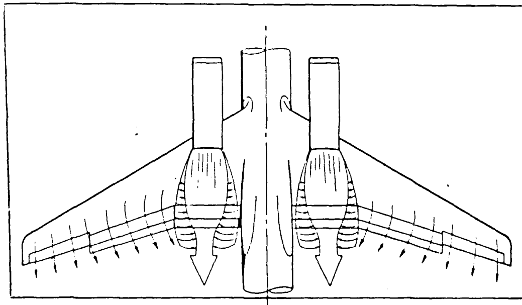
Figure 4.5 USB Flow Characteristics
