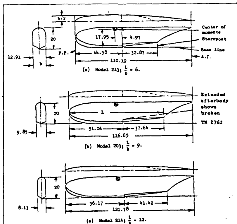
Figure 4.2 Some Flying Boat Hulls (NACA TN 1686)
