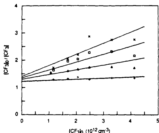
Figure 9. Reciprocal plot for determining the first- and second-order rate constants for the loss of \text{CF}_3 : 49 ms (X); 35 ms (□); 20 ms (Δ); 10 ms (+).
