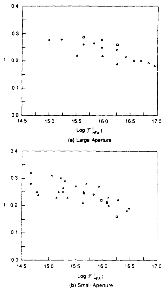
Figure 4. HFA depletion versus logarithm of the input flow for the large aperture (a) and the small aperture (b). The different symbols represent data taken on different days. The difference in the extent of the depletion on different days is due to changes in the output power of the photolysis laser.
