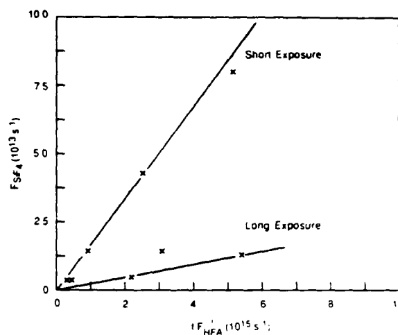
FIG. 5. SiF_4 production vs fF_{HFA} . The flow of HFA was varied and the depletion was constant at 15%. The temperature of the sample was 718 K. The data fall along two lines depending on whether the surface had been exposed for long ( \sim 90 min) or short times ( \sim 20 min).
