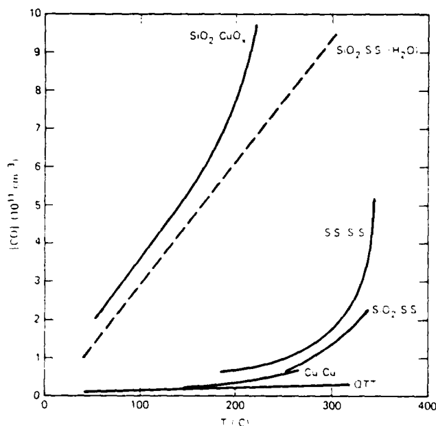
FIG. 4 CO concentration as a function of temperature for various substrates and heater assembly materials. Data taken with a stainless-steel heater with a silica substrate and without a substrate are labeled \text{SiO}_2/\text{SS} and \text{SS}/\text{SS} , respectively. Data taken with a clean copper heater and no substrate are labeled \text{Cu}/\text{Cu} . Data from an oxidized copper heater with a fused-silica substrate are labeled \text{SiO}_2/\text{CuO} . The dashed line, labeled \text{SiO}_2/\text{SS} (\text{H}_2\text{O}) , represents data from Selamoglu et al. (Ref. 11). The curve labeled QTT pertains to a quartz test-tube experiment. The flow rate in all these cases was \sim 4 \times 10^{11} \text{ molecule s}^{-1} . The laser depletion f was \sim 20\% for all cases, except for the dashed curve, where f was between 4\% and 14\% .
