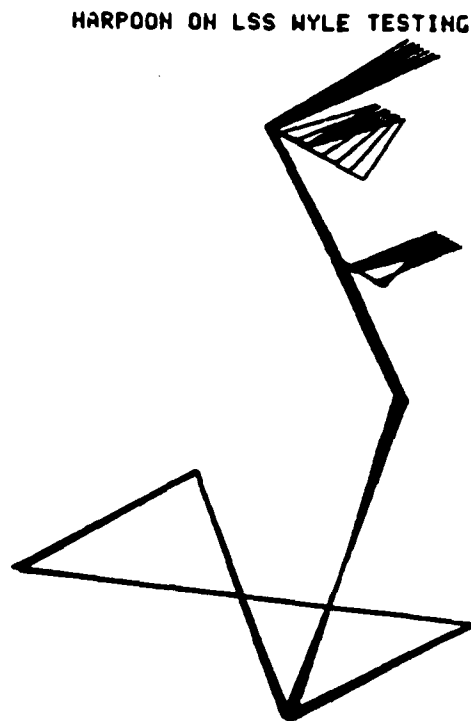
Figure 11.19 Y-Axis Input Mode Shape, 49.38 Hz, Modified Isolation Pads
