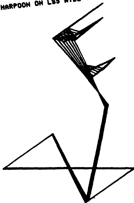
Figure 11.10 X-Axis Input Mode Shape, 23.75 Hz, Modified Isolation Pads
