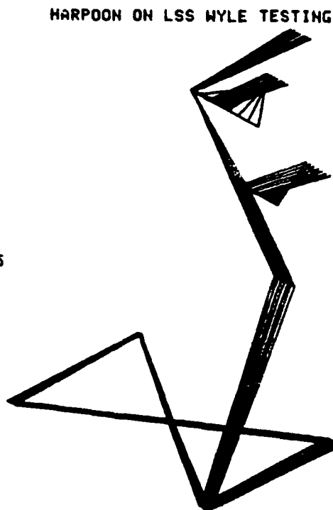
Figure 11.20 Y-Axis Input Mode Shape, 57.19 Hz, Modified Isolation Pads
