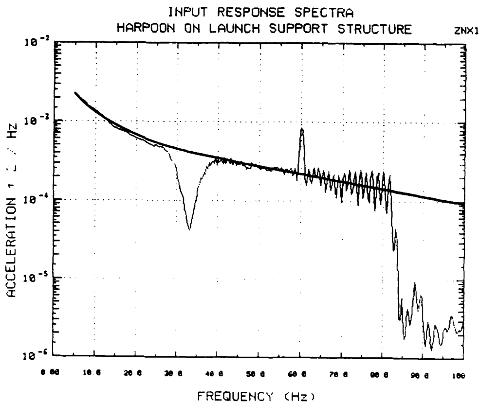
Figure 9.10 Z-Axis Input PSD with Modified Pads, Run No. 3
