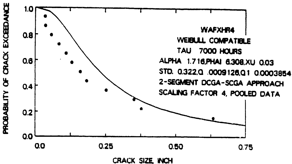
Figure 5-4. Correlation Between Predicted Crack Exceedance Probability at T = 11608 Flight Hours for WAFXMR4 Data Set and Actual Fractographic Results.
