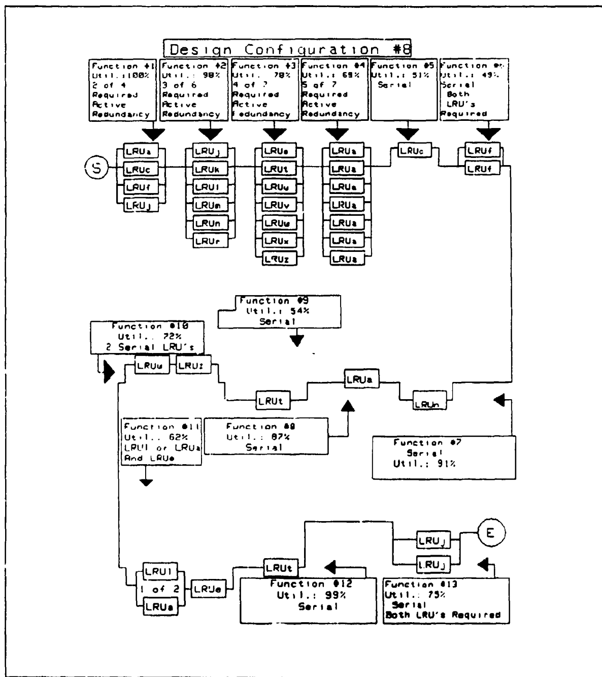
Figure 10 - Design Configuration #8's Reliability Block Diagram
