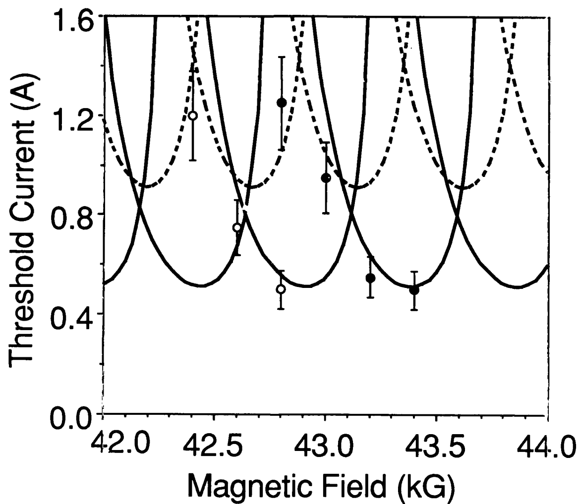
Figure 2. Threshold currents for the axial modes of resonator with 25 cm mirror separation and a gun voltage of 60 kV. Data for the 109.8 \pm 0.1 and 108.7 \pm 0.1 GHz modes is shown by the \bullet 's and \circ 's with error bars, respectively. Theoretical results as using \alpha = 1.5 are indicated by the solid and dashed curves.
