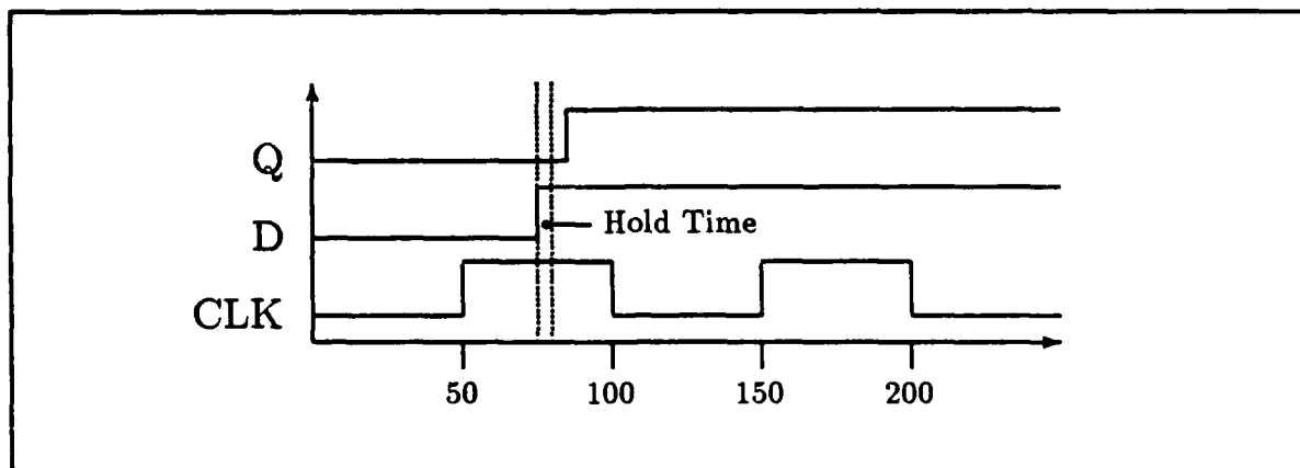
Figure 3-18. Hold Time
