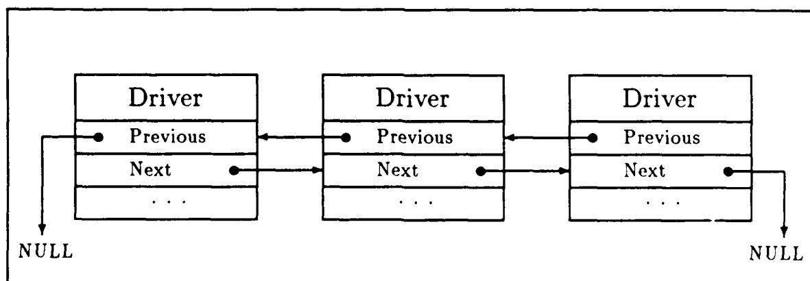
Figure 5-9. Event List
