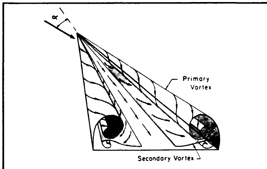
Figure 1. Vortical Flow Over a Delta Wing [1]
