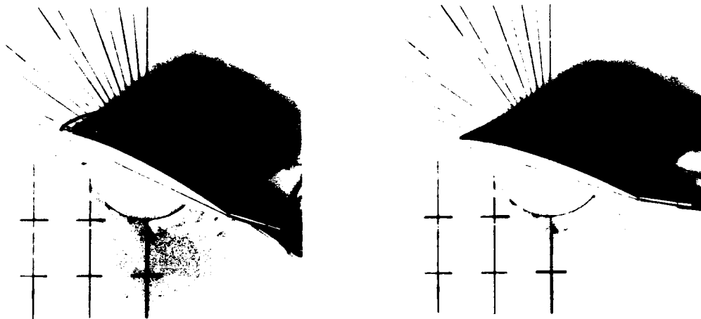
Figure 12. Examples of the Dynamic Stall Vortex Formed by the Rectangular Wing, \dot{\alpha}_{ND} = 0.2 Up and Down, Mid-Span, U = 0.6 in/sec
