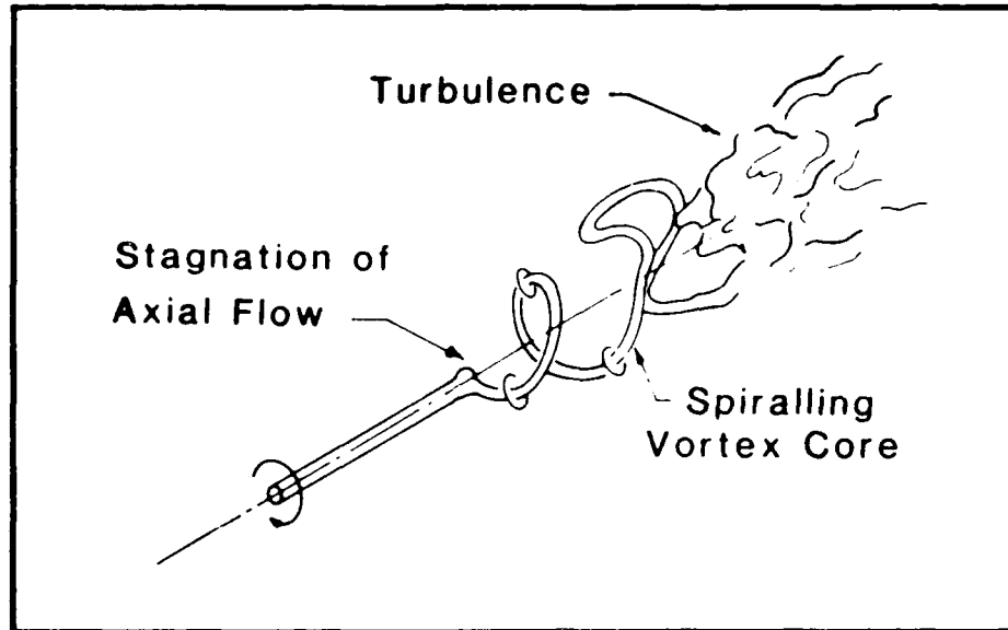
a. Spiral-Type Breakdown
