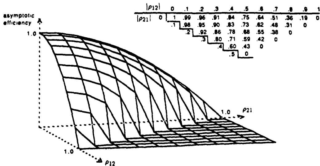
Fig. 22a. Asymptotic efficiency of the decorrelating detector for two users as a function of the partial crosscorrelations of their signature waveforms (recall |\rho_{12}| + |\rho_{21}| \leq 1 , and symmetry in \rho_{12}, \rho_{21} )
