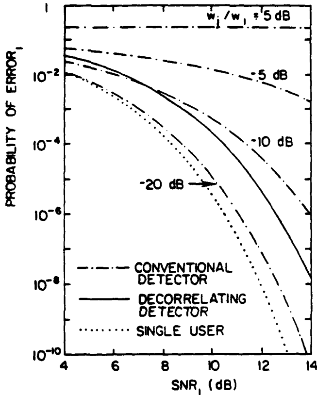
Fig. 1. Error probability of User 1 with 2 active equal energy interferers, each of energy w_j , averaged over the interfering bit sequences, for the decorrelating and conventional receiver versus the SNR of User 1, for m -sequences of length 31 and different interference levels.
