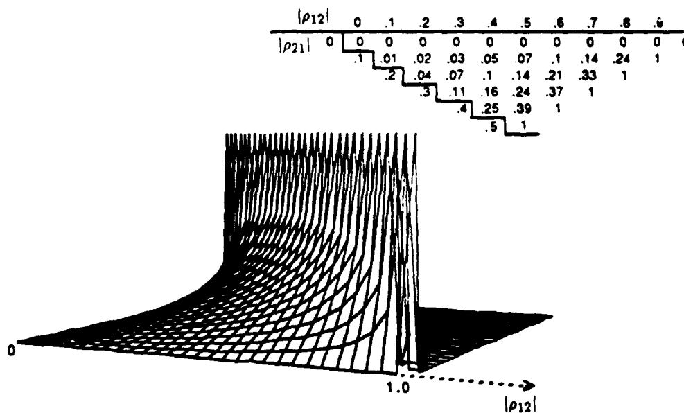
Fig. 22b. Decay rates of the coefficients of the IIR part of the decorrelating detector for two users, symmetric in \rho_{12} and \rho_{21} .
