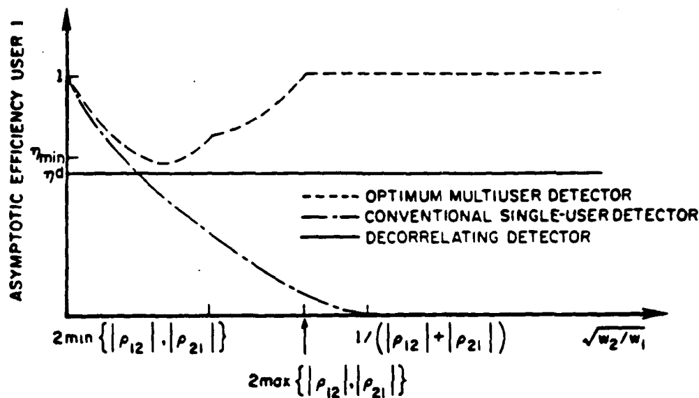
Fig. 20. Asymptotic efficiencies in the 2-user case for infinite transmitted sequence length, when the user energies are constant over time (here we chose |\rho_{12}|, |\rho_{21}| = 0.3, 0.5 which yields \eta_{min} = 0.68 , \eta^d = 0.59 ).
