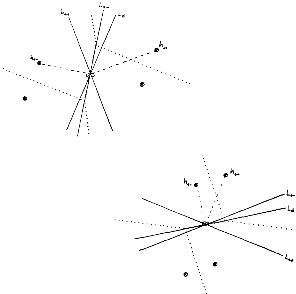
Fig. 8. Geometric illustration of Proposition 3.9.
