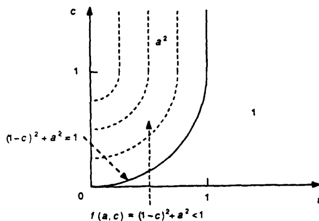
Fig. 10. Function f(a, c) of Proposition 3.17.
