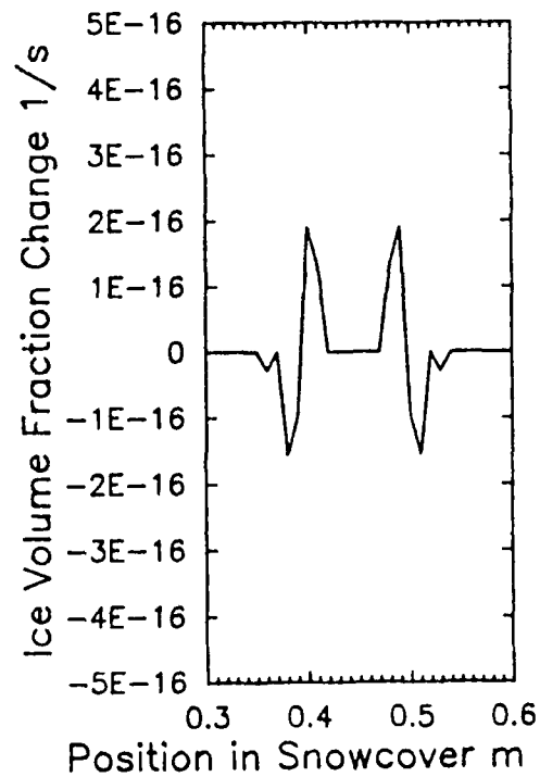
Figure 11. Vapor flux and condensation rate in layered snow cover with uniform temperature distribution.
