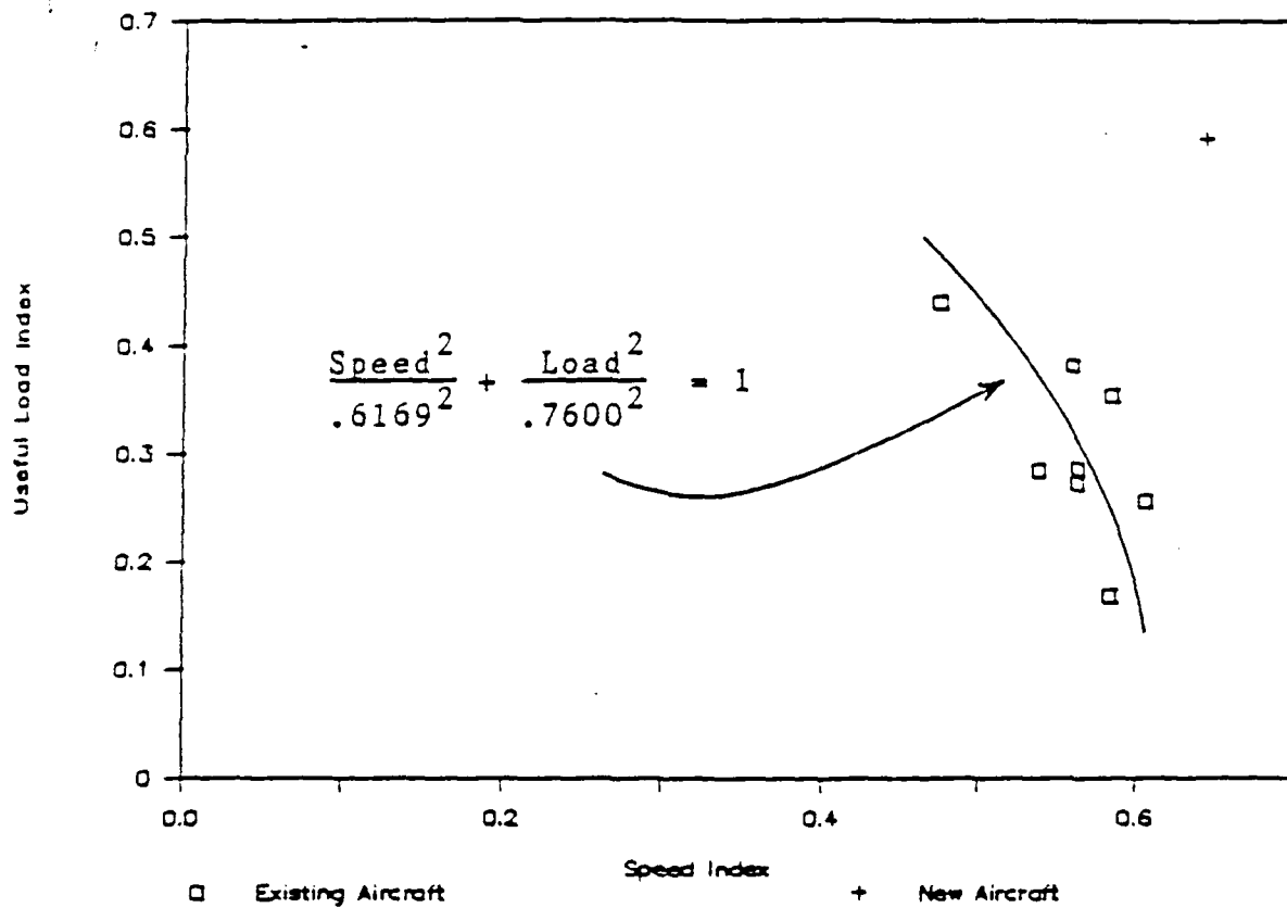
Figure 1 ELLIPSOID METHOD Aircraft Speed versus Useful Load
