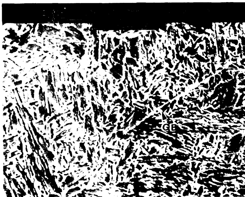
Figure 20. SEM Micrograph of Sample W6 (Low Hardness)
