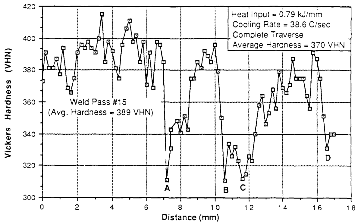
Figure 7. Microhardness Profile for W58
