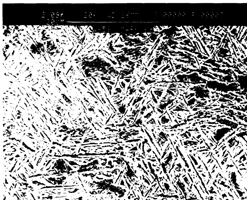
Figure 26. SEM Micrograph of Sample W58 (High Hardness)
