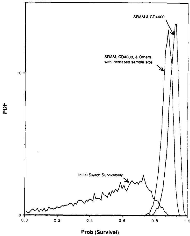
Figure 2 Calculated 5ESS Survivability at 500-1k Rads
