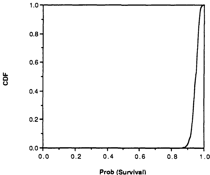
CDF Survival Curve for 4k/16k SRAM, 500-1k Rads(Si) Bin (113 survivals out of 119 samples)
