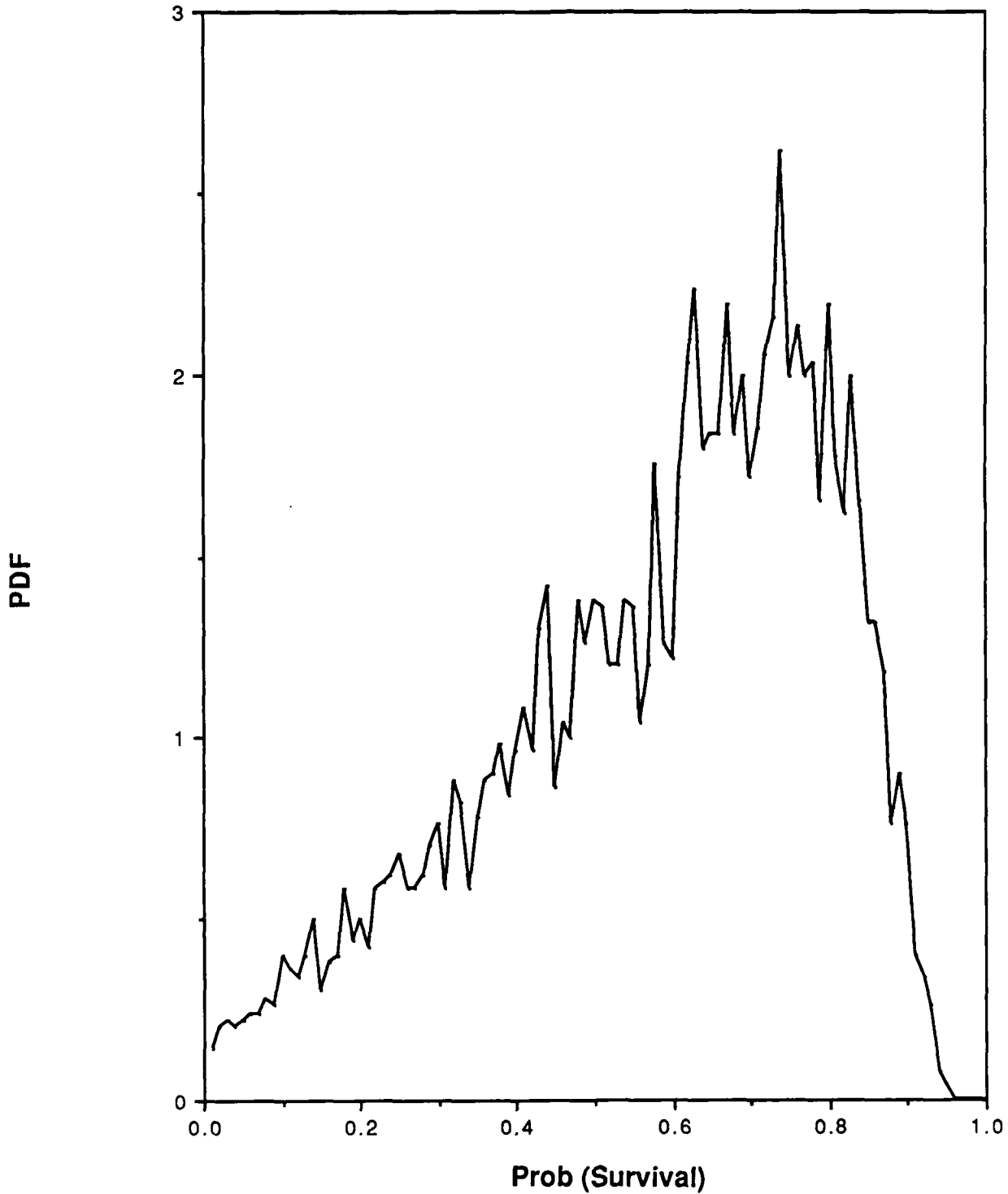
PDF Survival Curve for the 5ESS Switch, 0-500 Rads(Si) Bin
