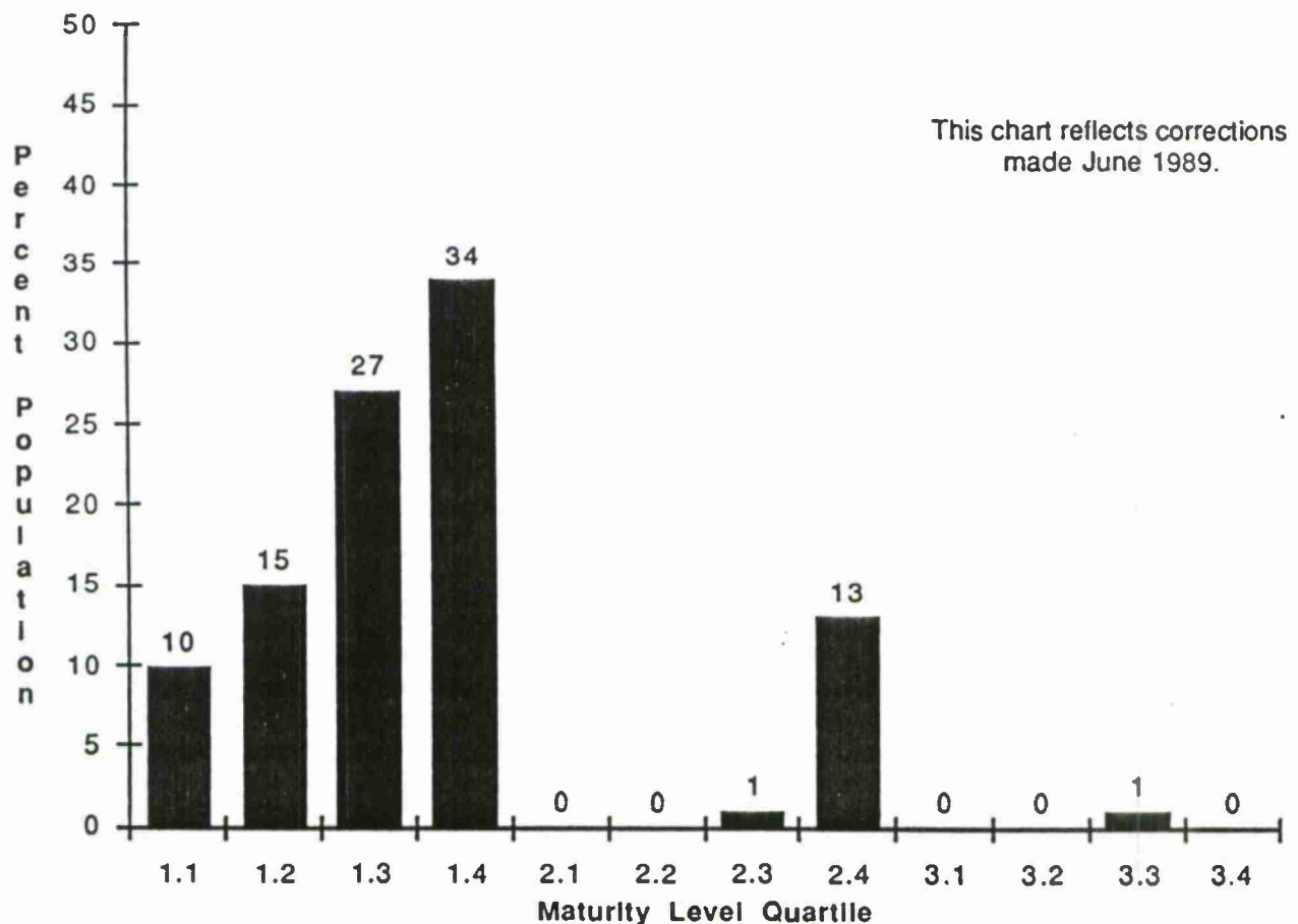
Figure 2.3.1.1: Software Process Maturity Level Distribution - Workshop Assessment Data (113 Data Points) 7
