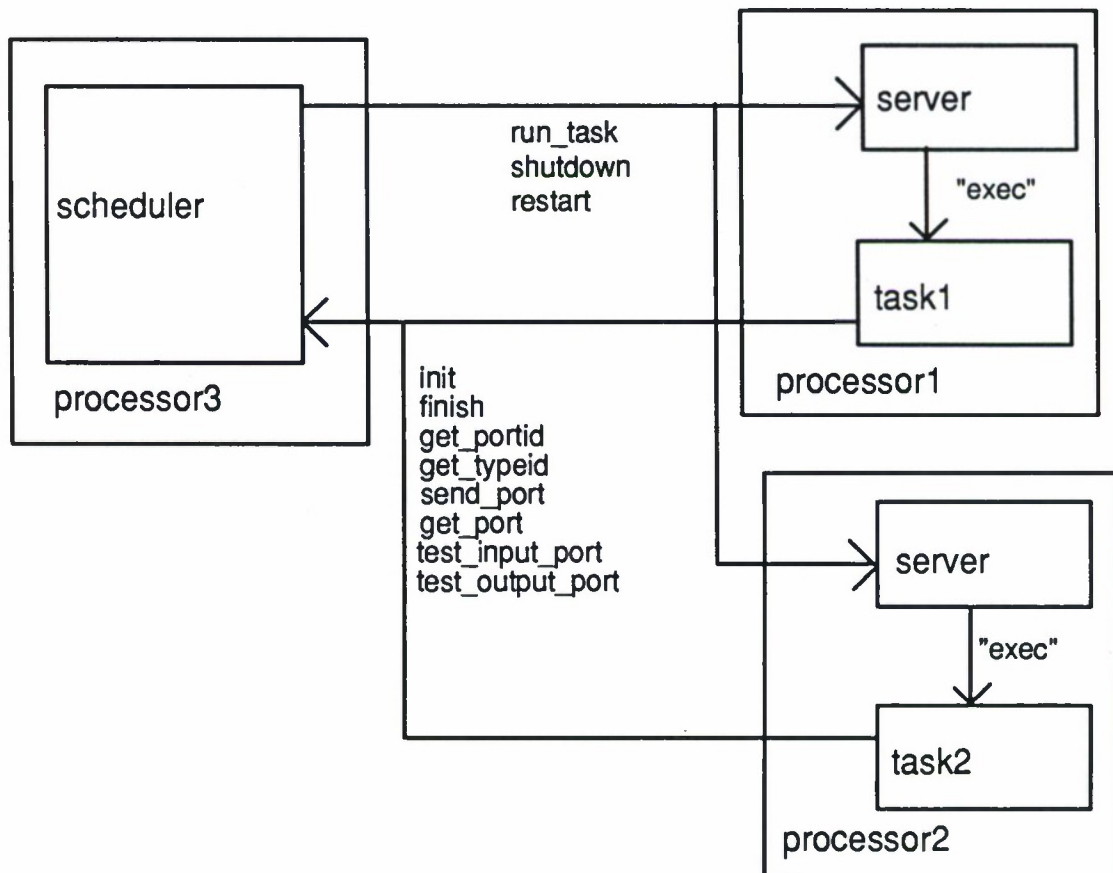
Figure 1-6: The Durra Runtime Environment
