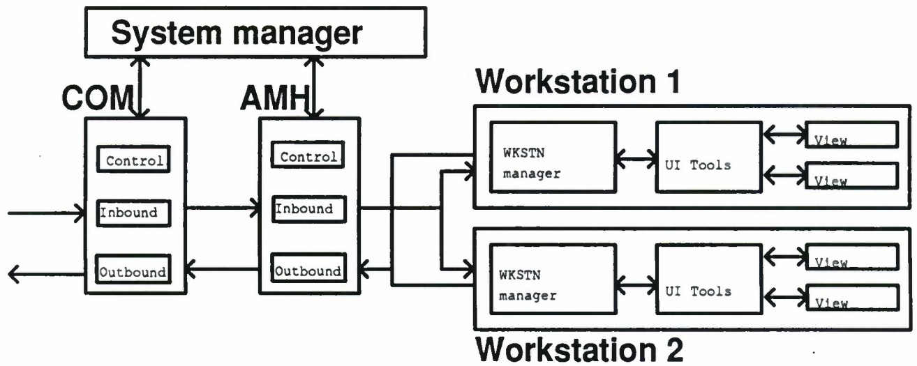
Figure 4-3: Final Structure of the C 3 I Node
