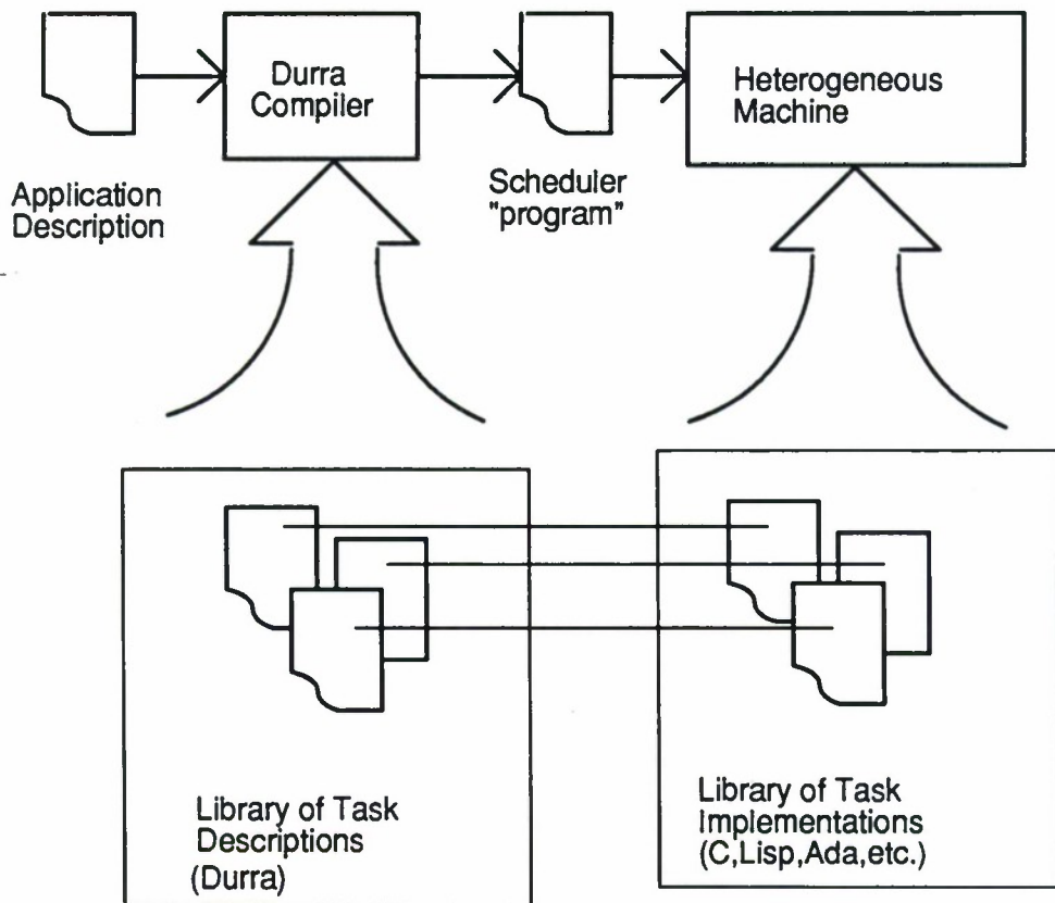
Figure 1-5: Scenario for Developing an Application in Durra
