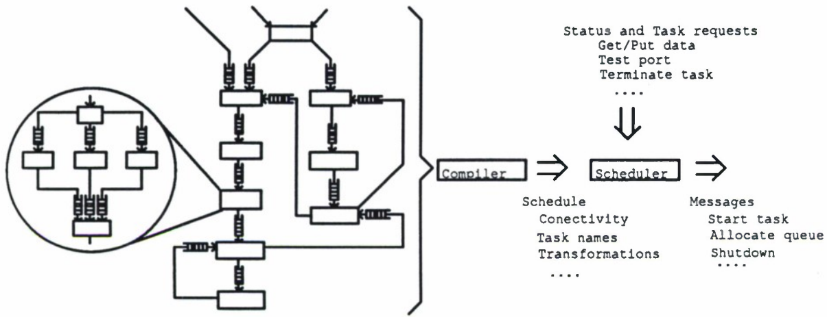
Figure 1-1: Compilation of an Application Description
