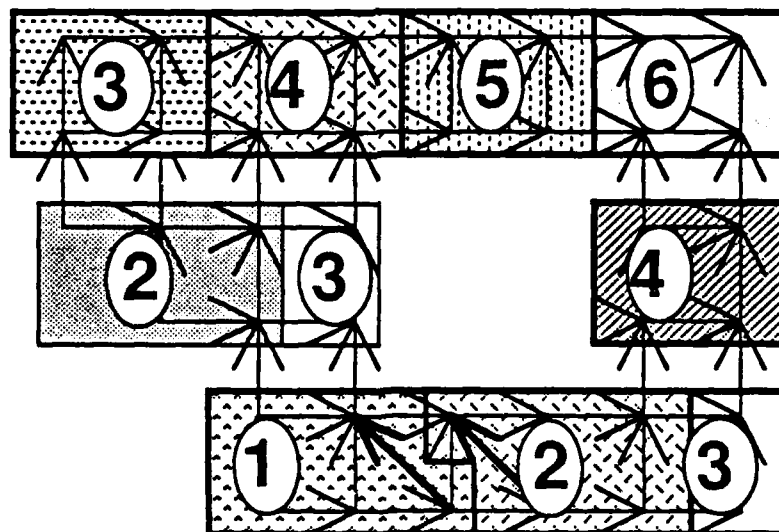
Figure 9: Disadvantageous Cluster DAG for Irregular Problem
