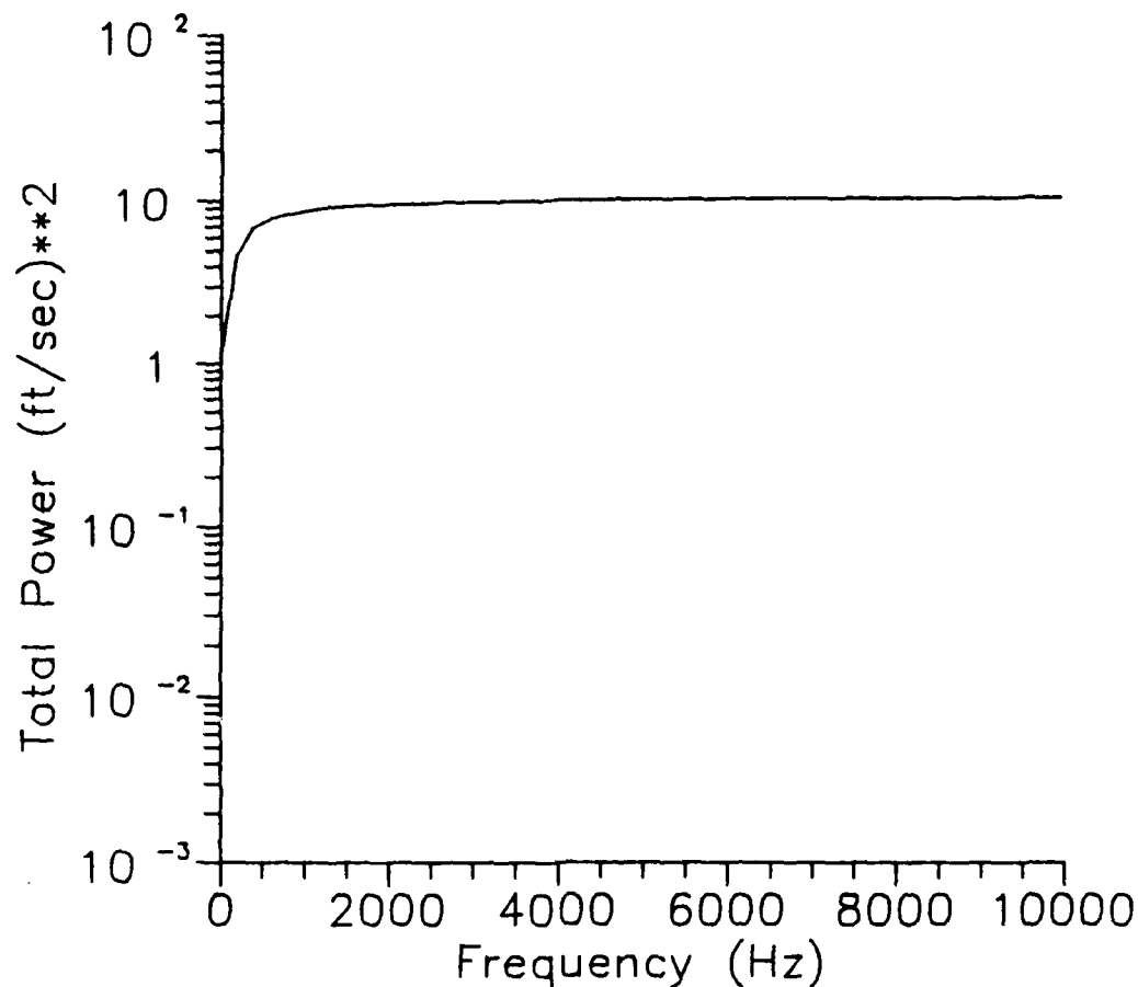
Figure 27. Total Power Distribution for Test Case A, Turbulence Pulse
