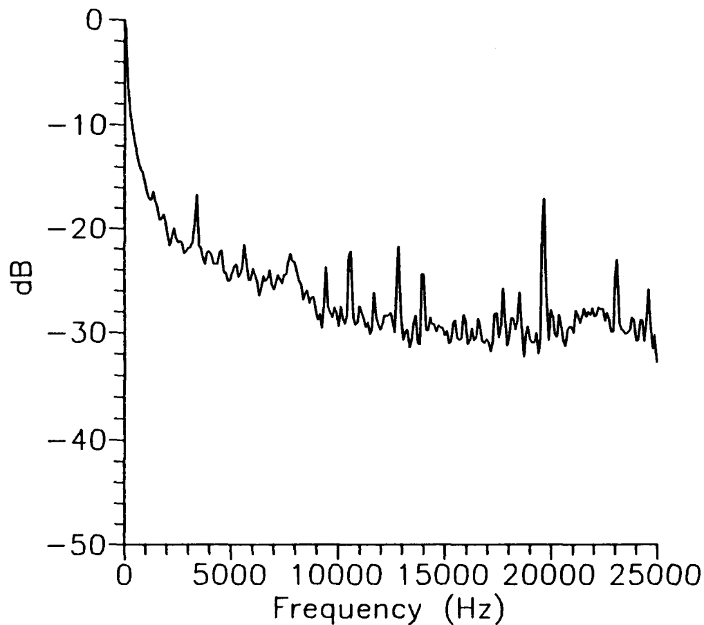
Figure 29. Free Stream Velocity Spectrum
