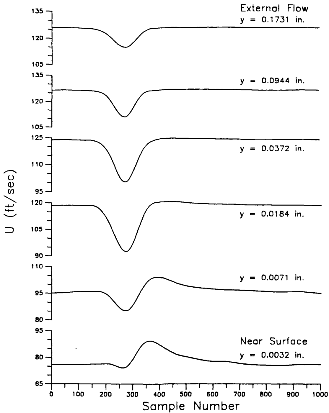
Figure 36. Mean Velocity Time Histories in the Boundary Layer, 30% Chord: ( F_s = 50 KHz)
