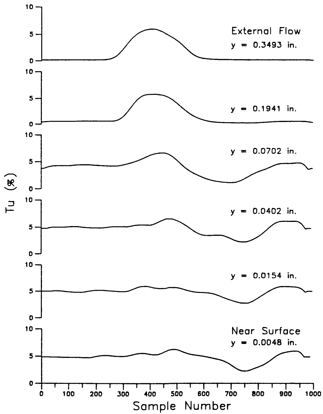
Figure 54. Mean Turbulence Time Histories in the Boundary Layer, 70% Chord: ( F_s = 50 KHz)
