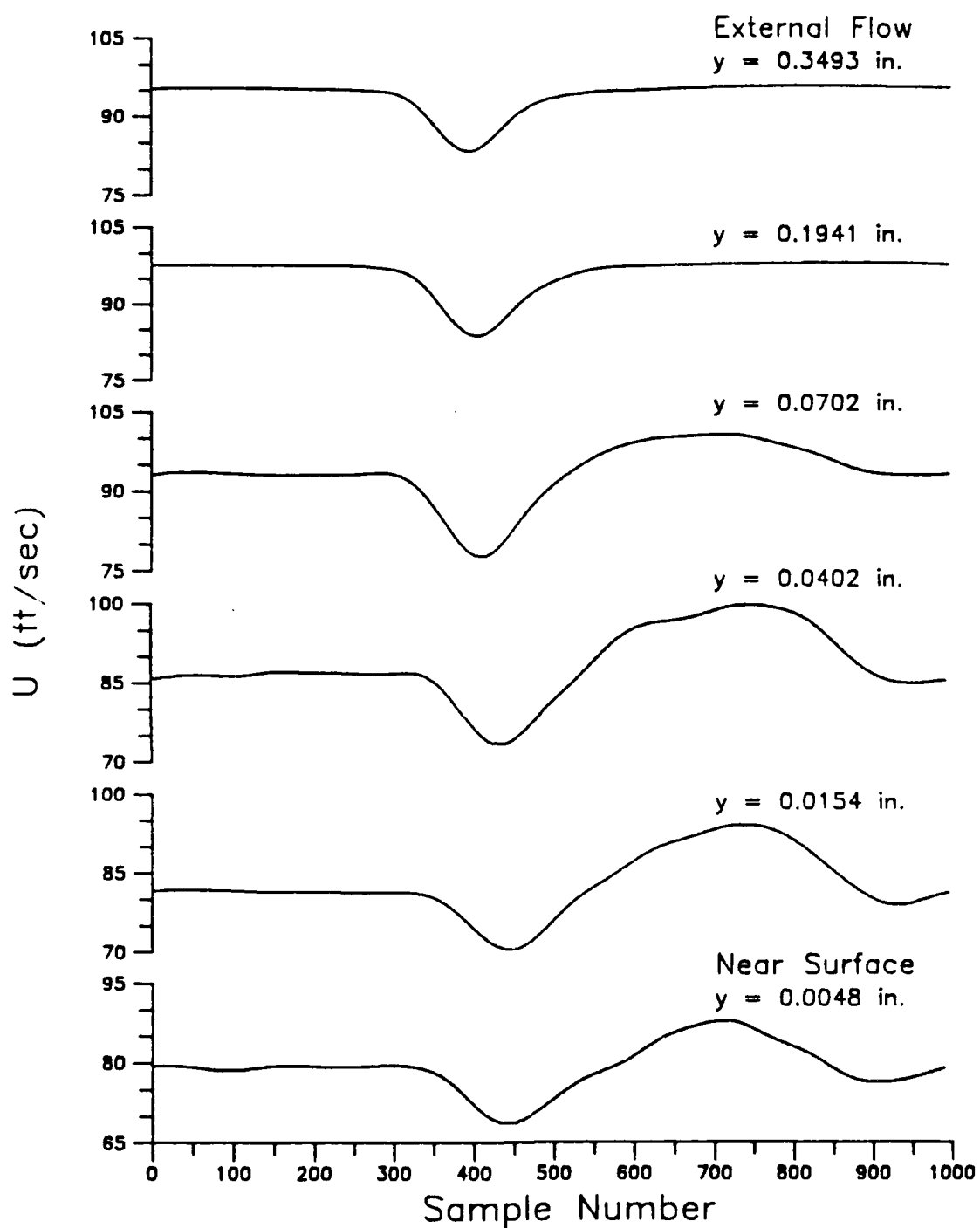
Figure 53. Mean Velocity Time Histories in the Boundary Layer, 70% Chord: ( F_s = 50 KHz)
