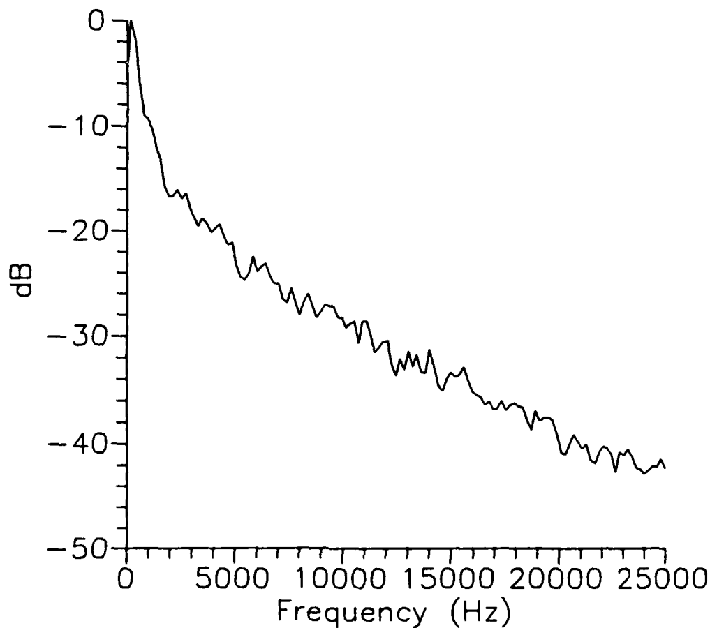
Figure 26. Velocity Spectrum for Test Case A, Turbulence Pulse
