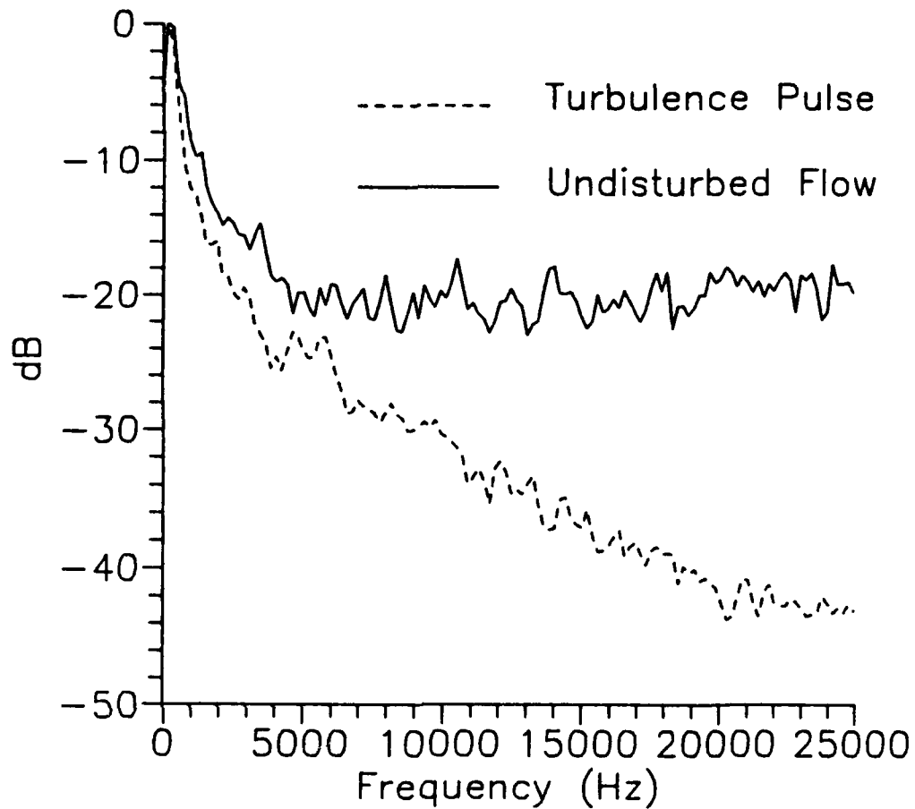
Figure 33. Turbulence Pulse Velocity Spectrum
