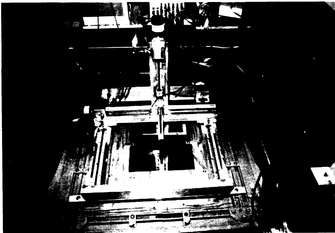
Figure 9. 3-D Traverser
