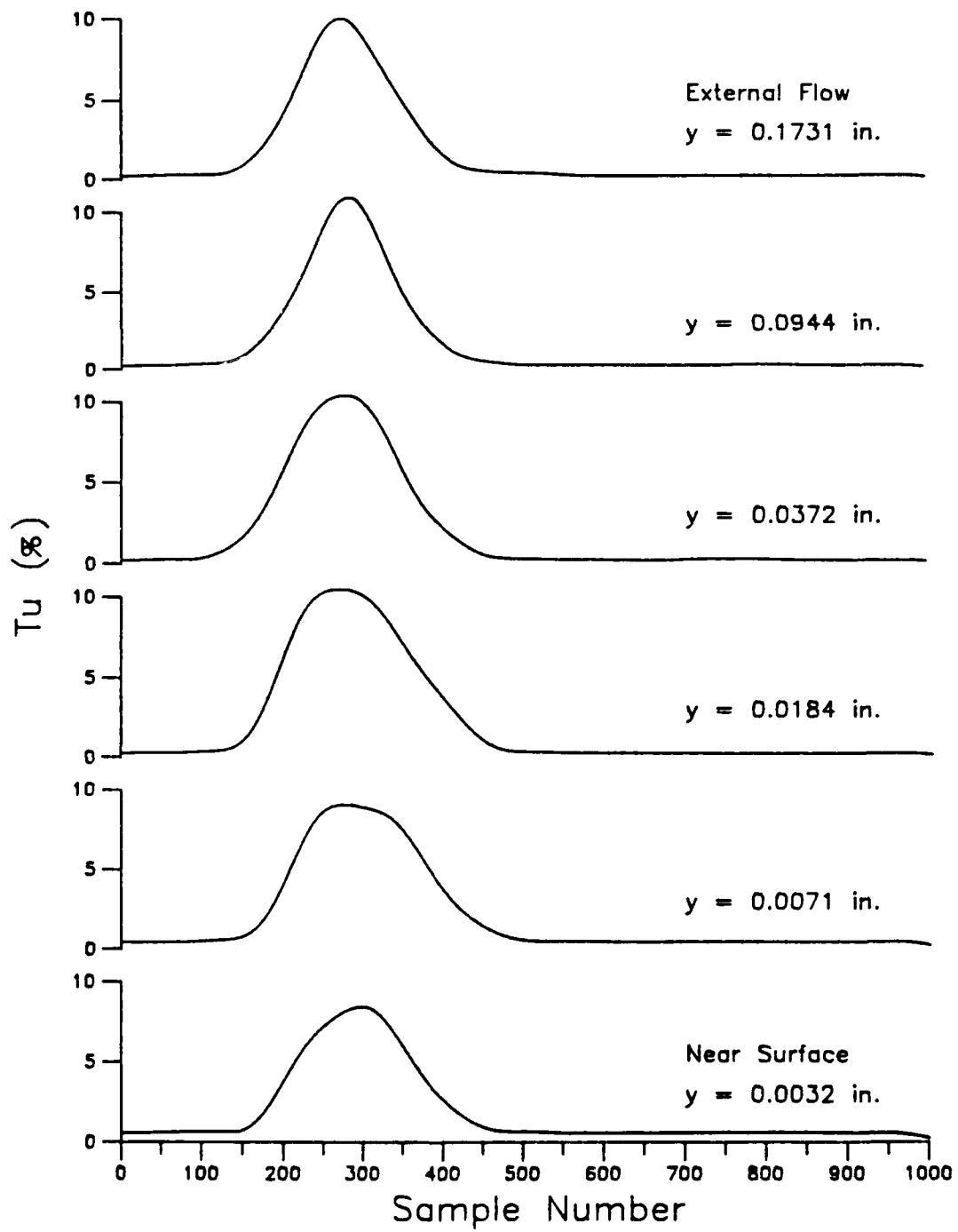
Figure 37. Mean Turbulence Time Histories in the Boundary Layer, 30% chord: ( Fs = 50 KHz)
