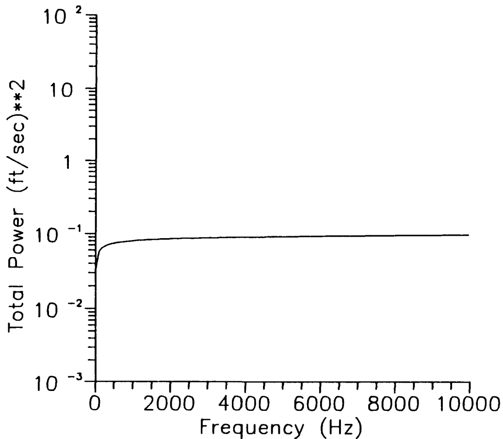
Figure 30. Free Stream Total Power Distribution
