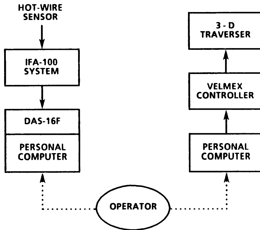
Figure 13. Equipment Configuration
