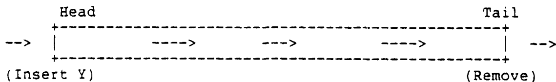
Figure 5.12 FIFO Queue
