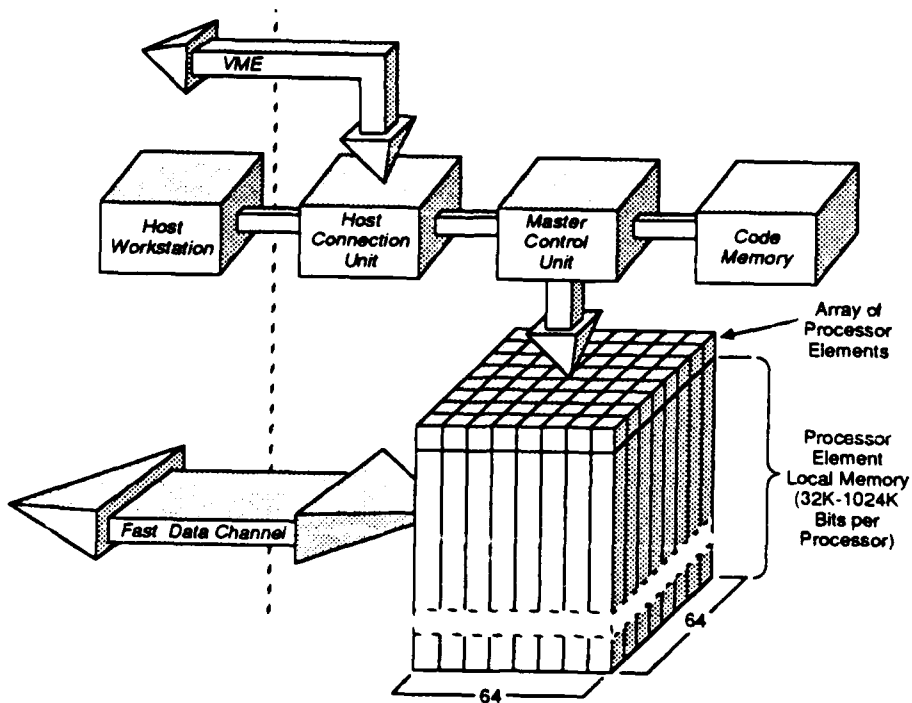
Figure 3. Major Functional Units of the DAP 610
